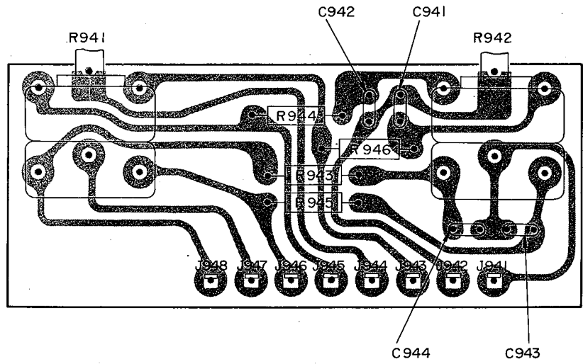
Figure 14 Tone Control Unit Assembly P940 Component Locations.
