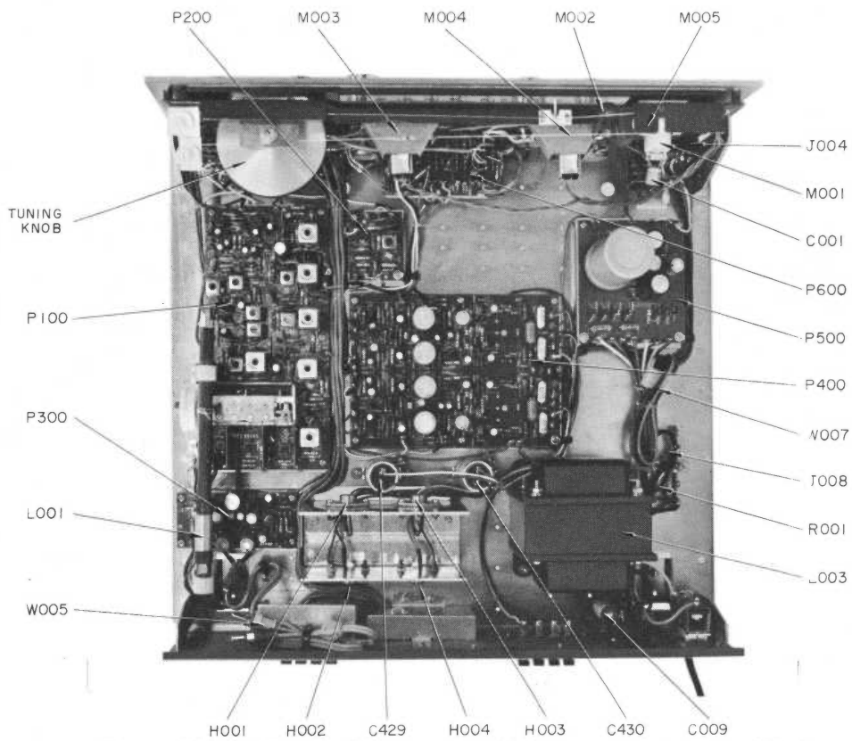
Figure 2 Main Chassis Adjustment and Component Locations (Top)
