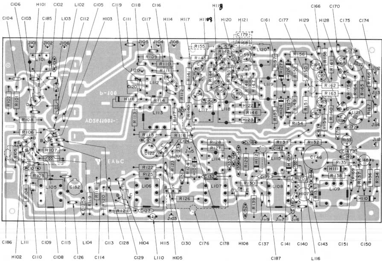
Figure 5 AM/FM/FM MPX Tuner Circuit
