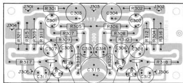
Figure 7 PONO Amplifier
