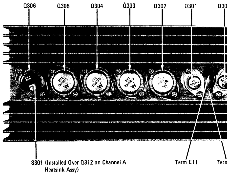
Channel B Heatsink Assembly Shown (Same as Channel A Except as Noted)
