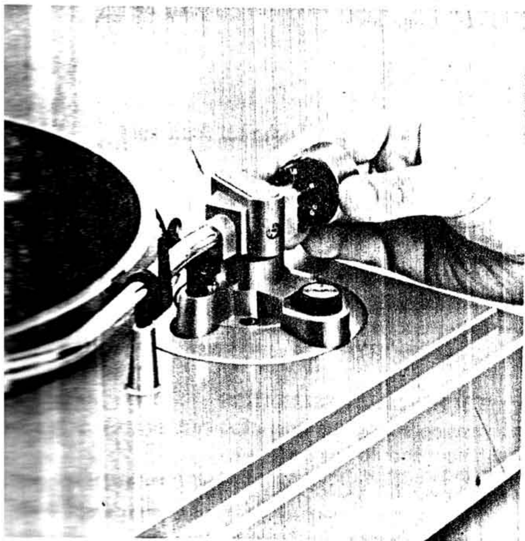
Figure 3. Anti-Skating Mechanism
