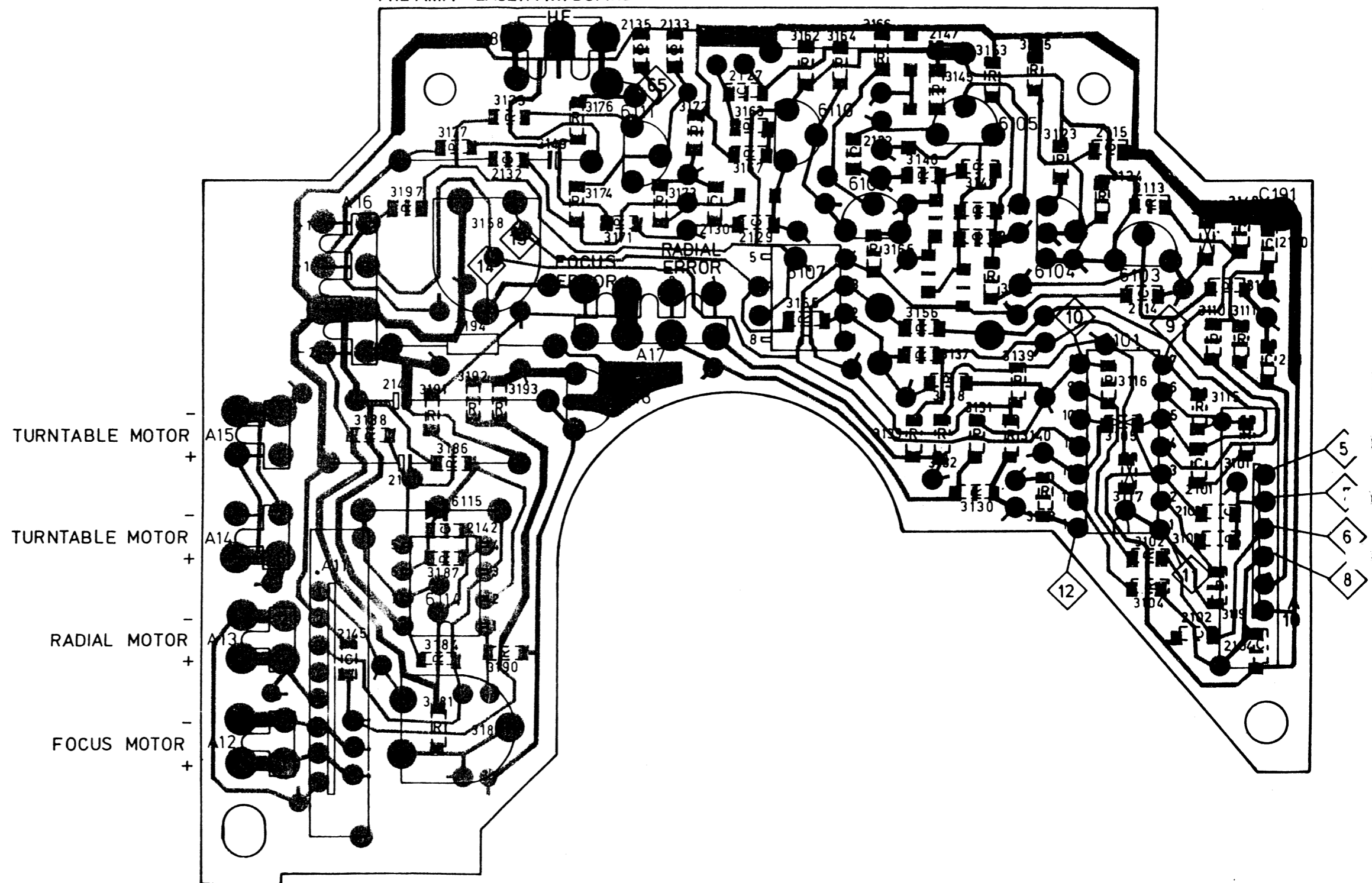
PRE AMP. + LASER P.W. BOARD
