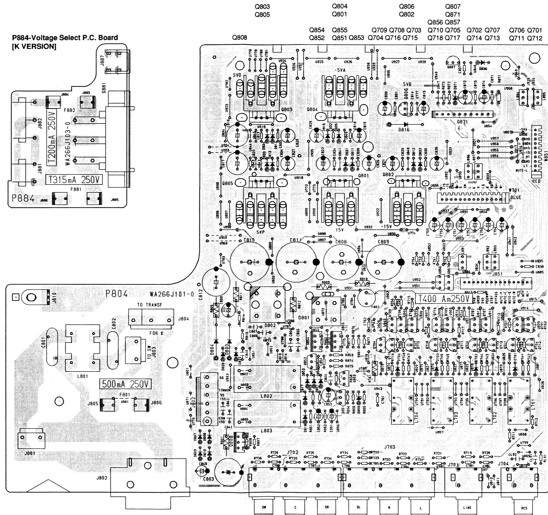
P804-Power P.C. Board
