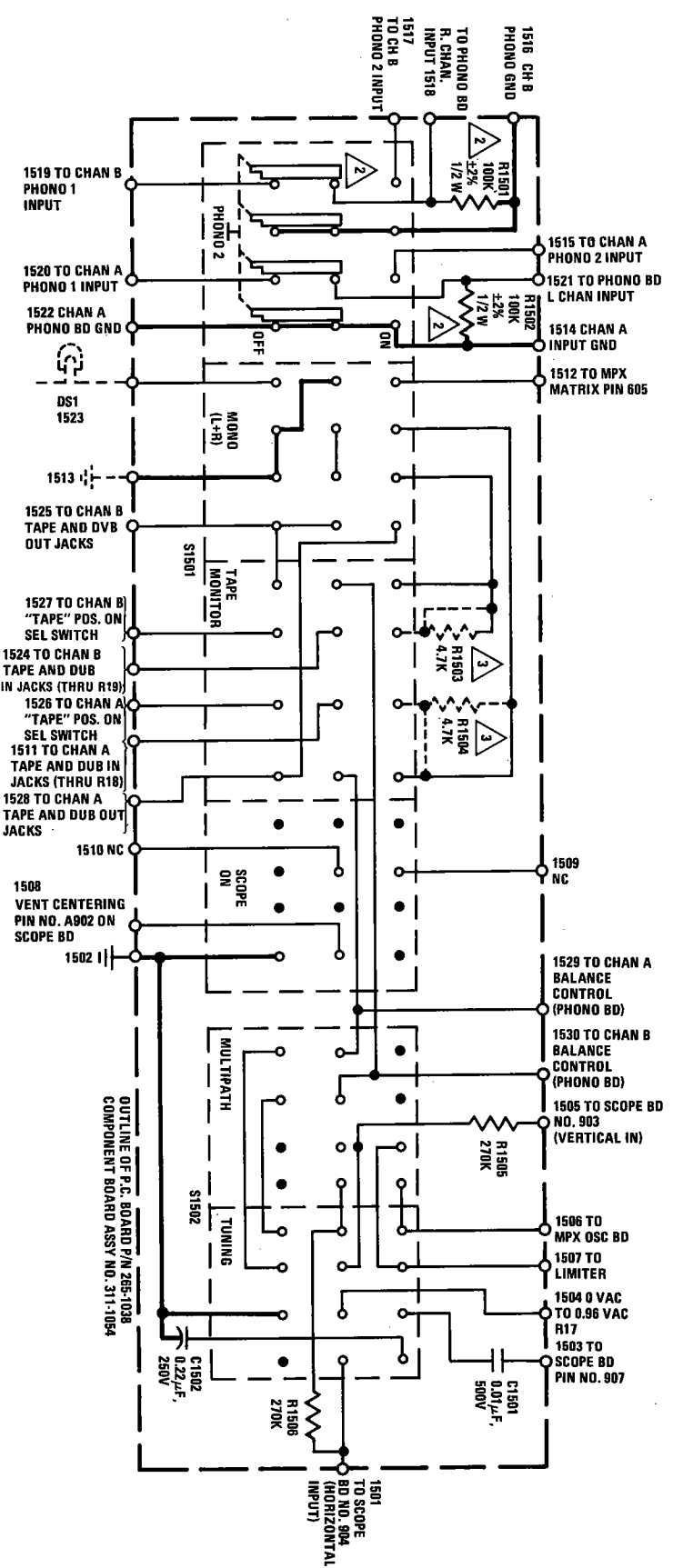
FIGURE 21A - FUNCTION SWITCH SCHEMATIC DIAGRAM
