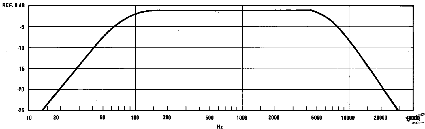
FIGURE 22D – HI-LOW FILTER CURVE
