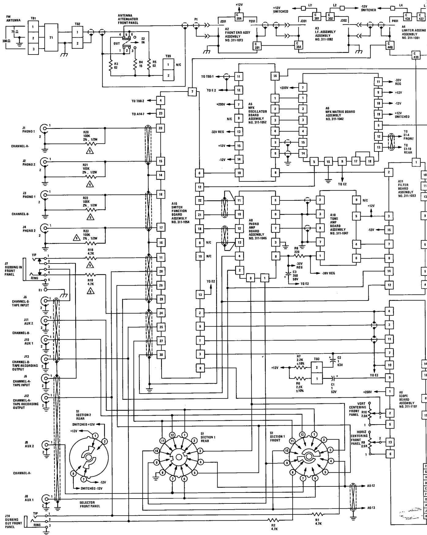
FIGURE 24 - MODEL 19 UNIT SCHEMATIC
