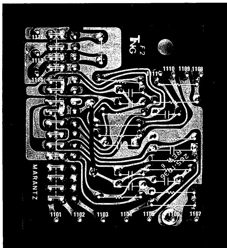
FIGURE 22B – HI-LOW FILTER (OLD) CONDUCTOR DIAGRAM
