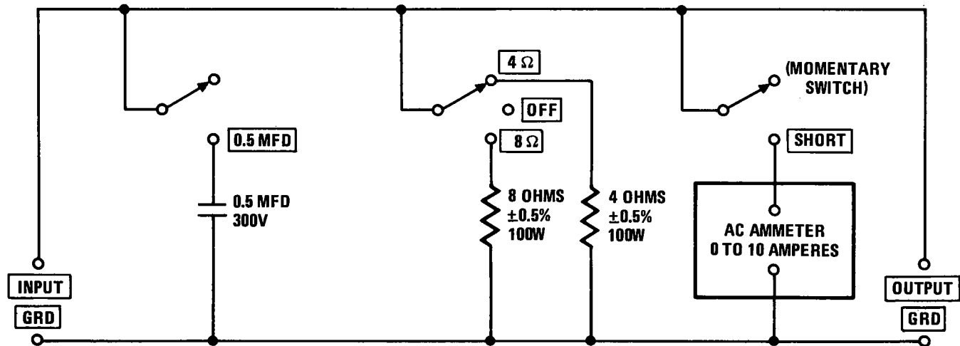
FIGURE 2 – AMPLIFIER OUTPUT LOAD BOX SIMPLIFIED SCHEMATIC
