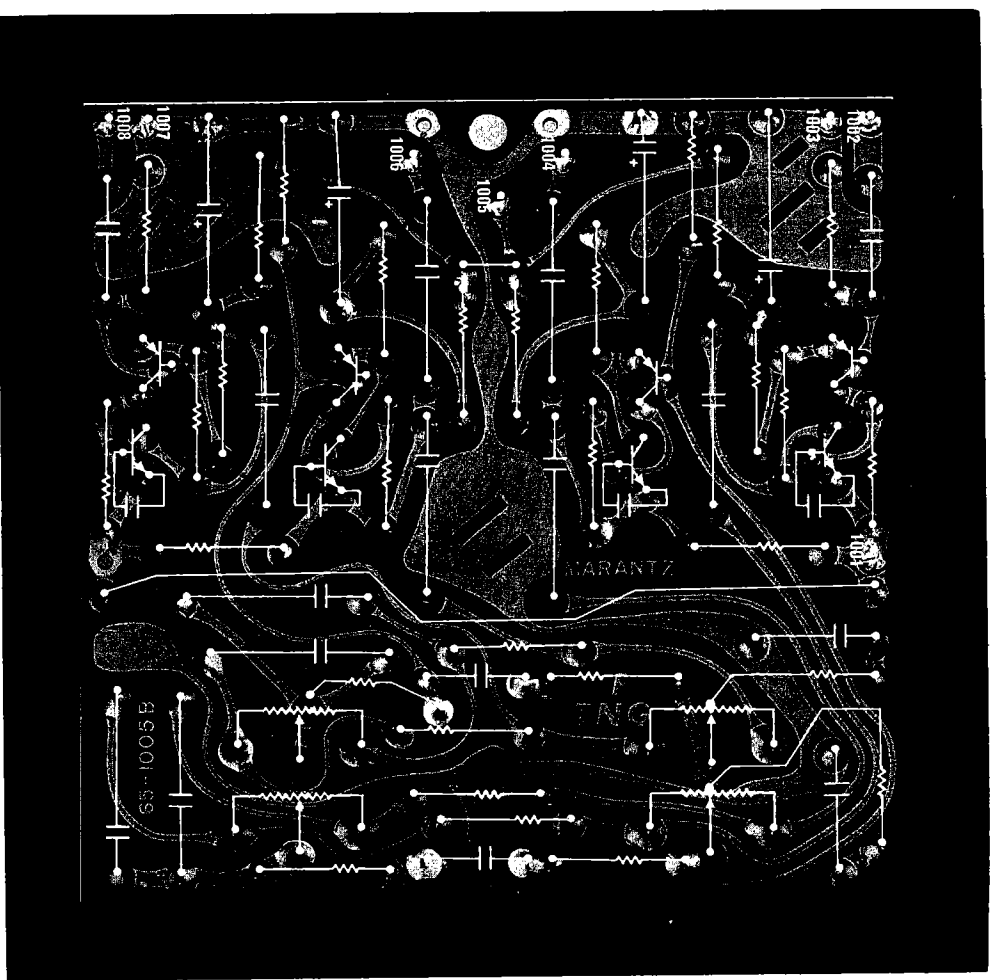
FIGURE 16B - TONE CONDUCTOR DIAGRAM
