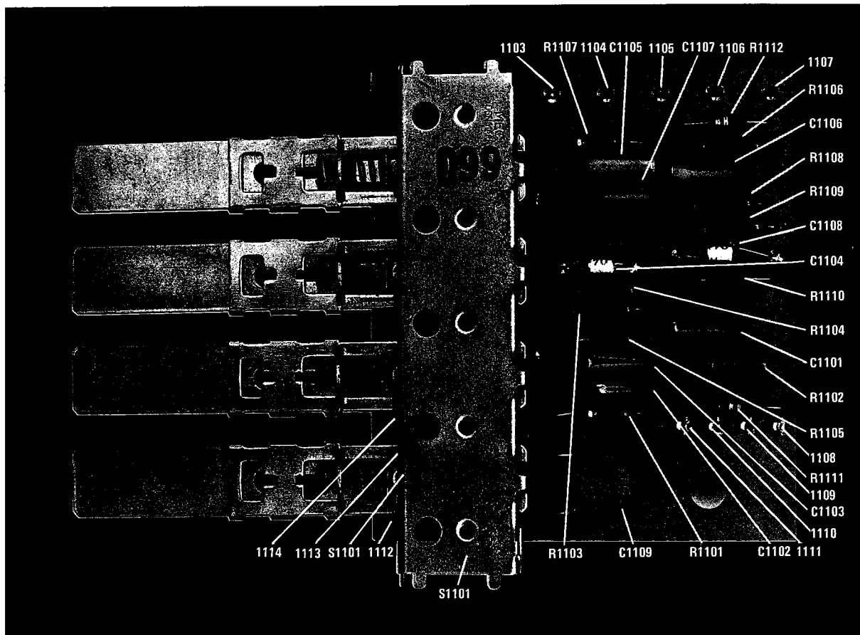
FIGURE 22A – HI-LOW FILTER (OLD) COMPONENT DIAGRAM
