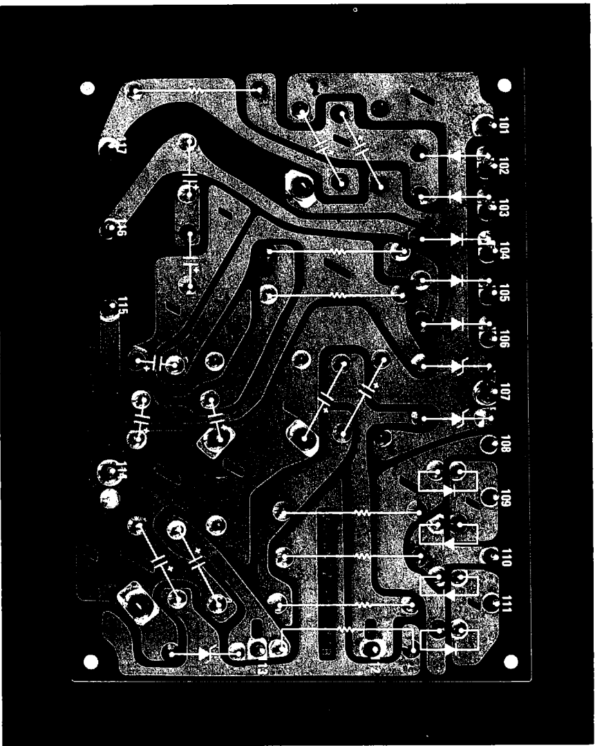
FIGURE 7B - POWER SUPPLY CONDUCTOR DIAGRAM
