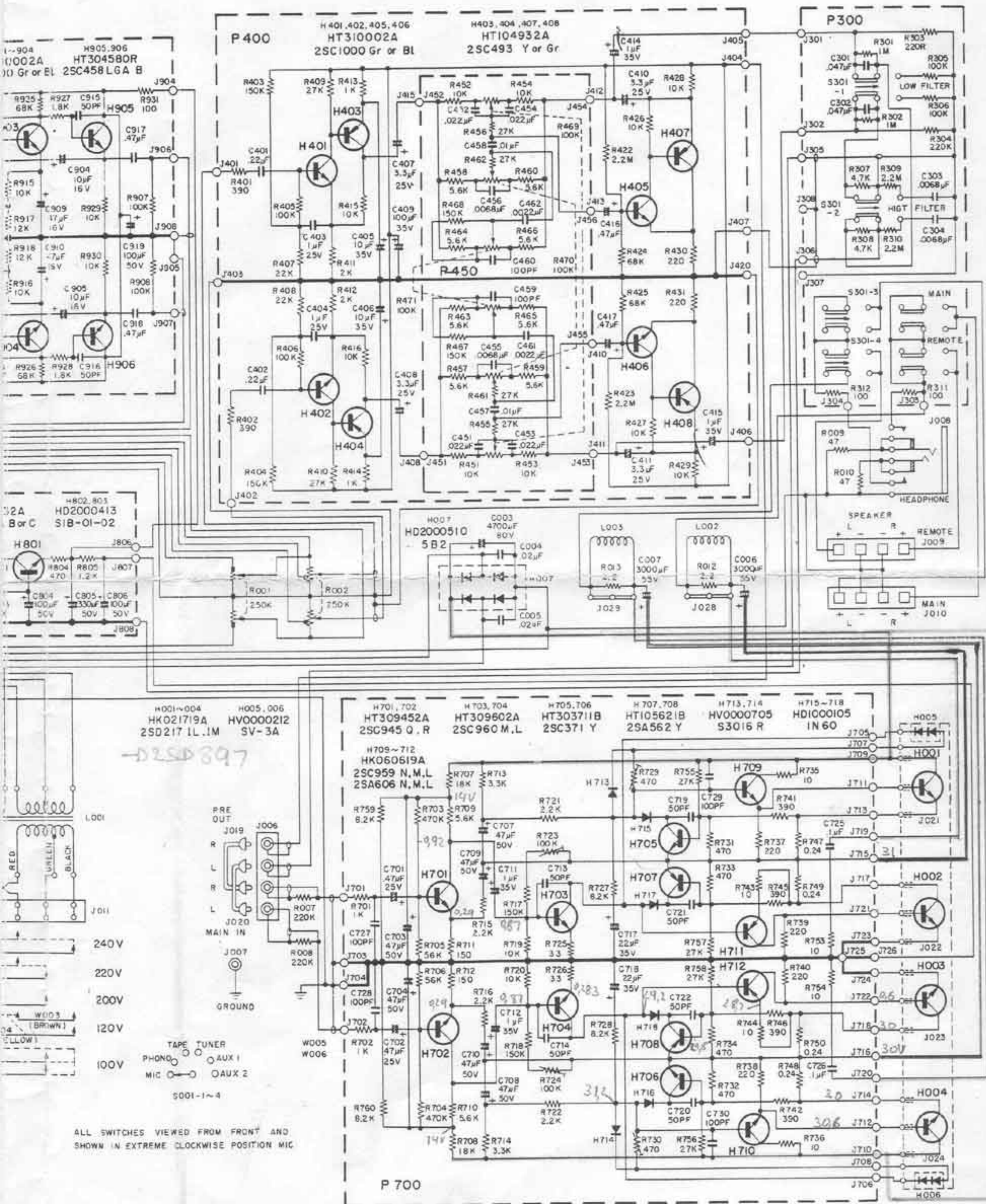
Figure 16. Schematic Diagram
