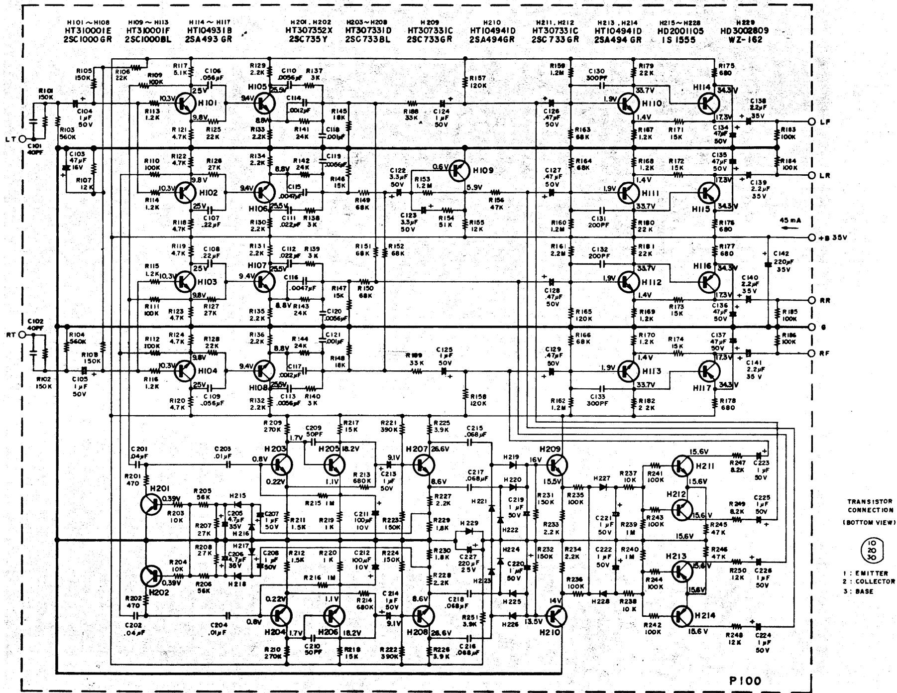
Marantz SQA 1 - Schematic Diagram
