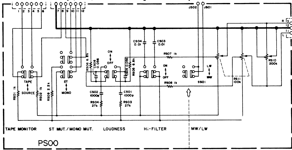
5.5 Switch Assembly (PS00) Schematic Diagram and Component Locations
