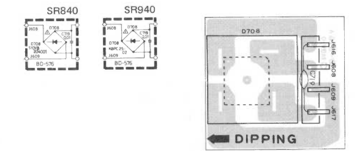
6.13 Rectifier (BD-576) Schematic Diagram and Component Locations
