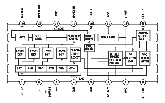
IC12 : LA1235
