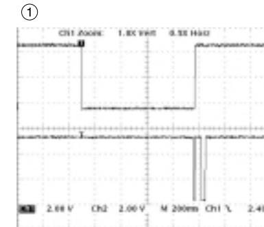
TURN(+)(-) Signal from \mu -com
