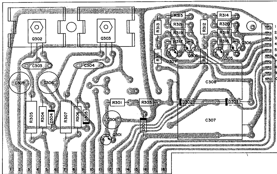
POWER SUPPLY PC BOARD O44-964
