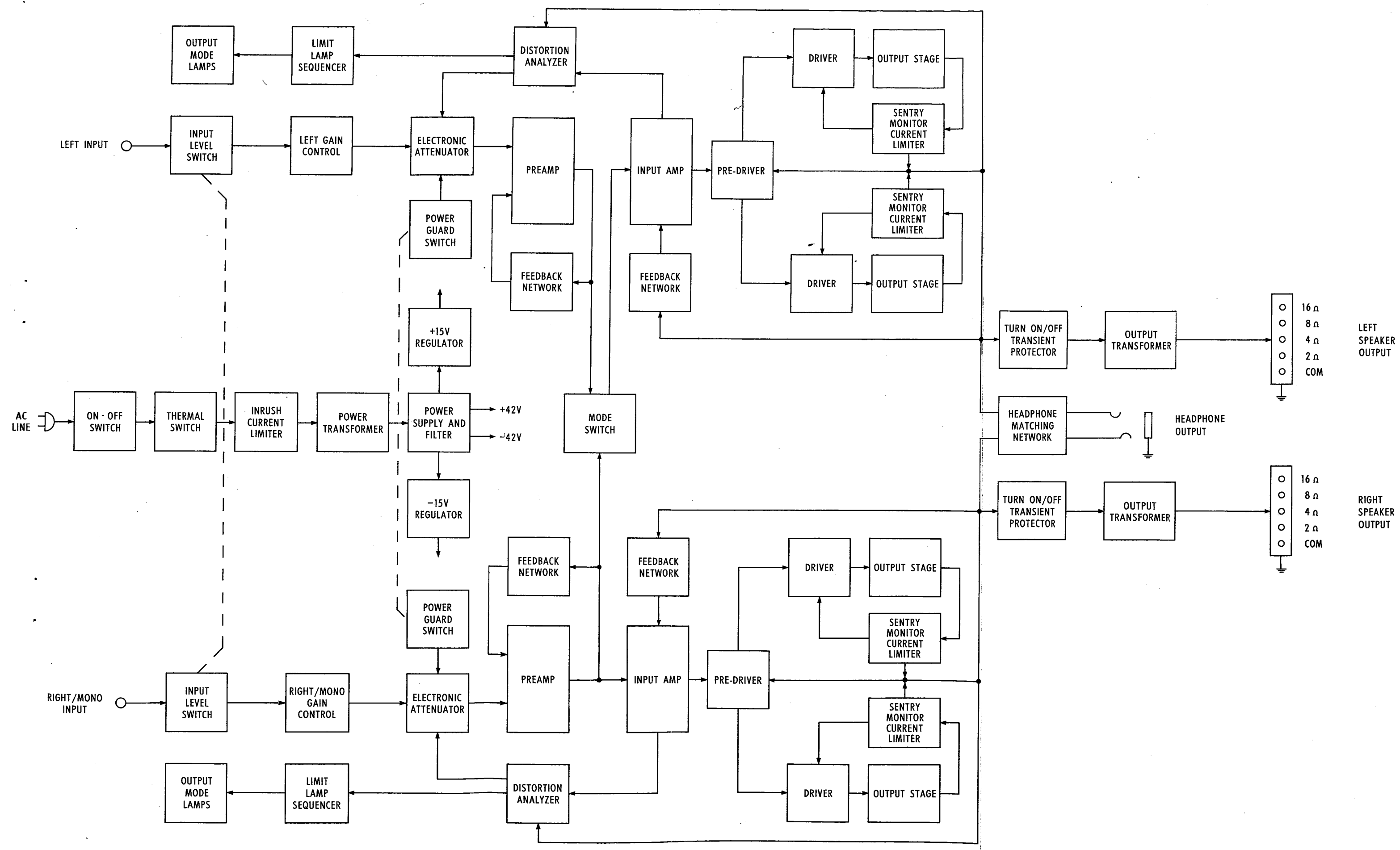
BLOCK DIAGRAM
