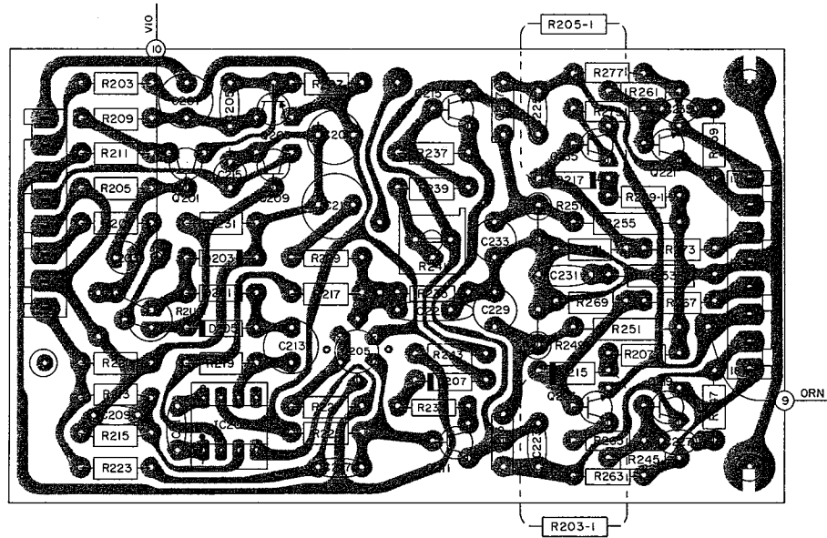
LEFT CHANNEL POWER OUTPUT PC BOARD O44-626
