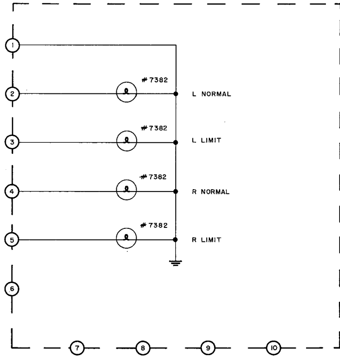
LIMIT LAMP PC BOARD 044-965
