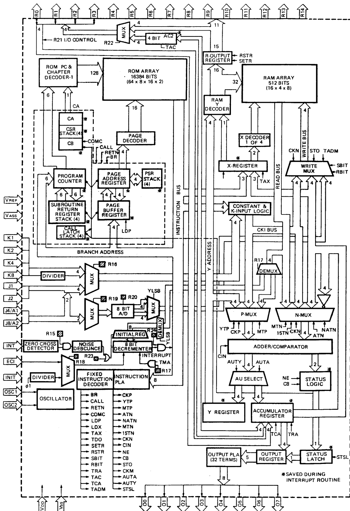
MP9457: IC201 (2/2)
