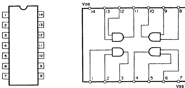
TC4081BP: IC401
