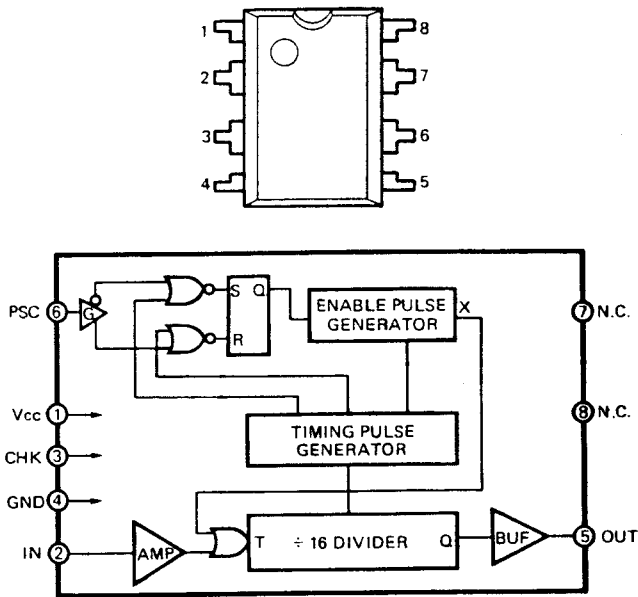
\mu PB553AC: IC103
