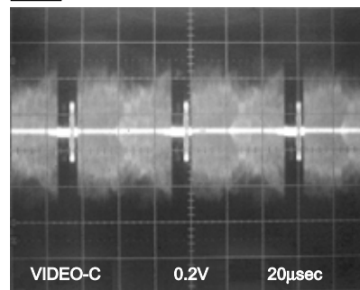
WF2 Pin 9 of CN1601
