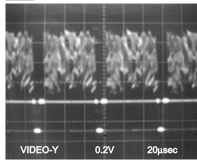
WF1 Pin 7 of CN1601
