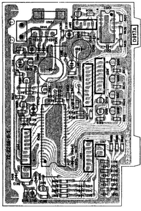
\mu COM P.C.B. ASS'Y (D017A)
