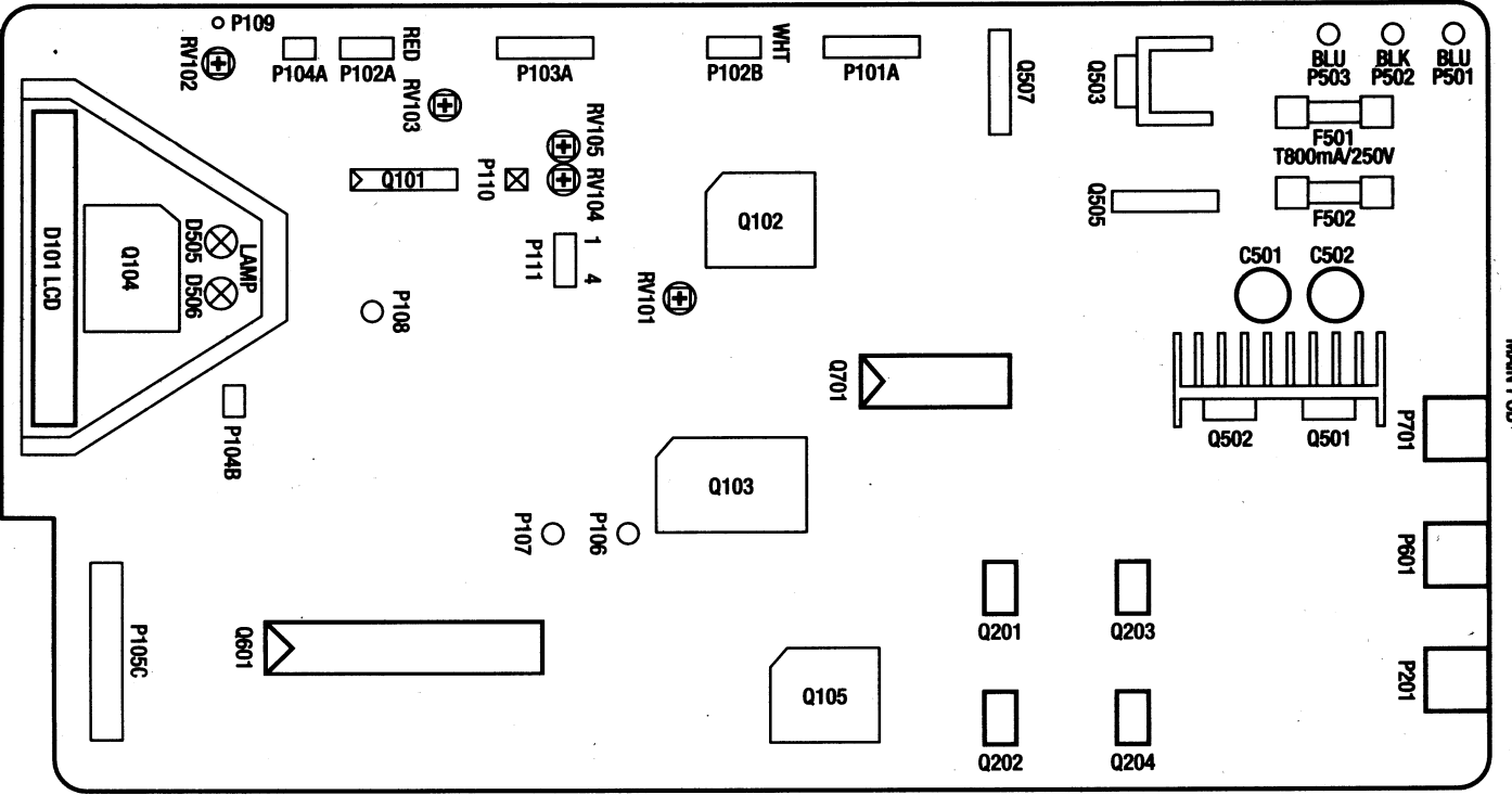
NAD - 512 PCB ADJUSTMENT POINTS DIAGRAM
