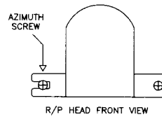
Fig. B FOR ADJUSTING AZIMUTH
