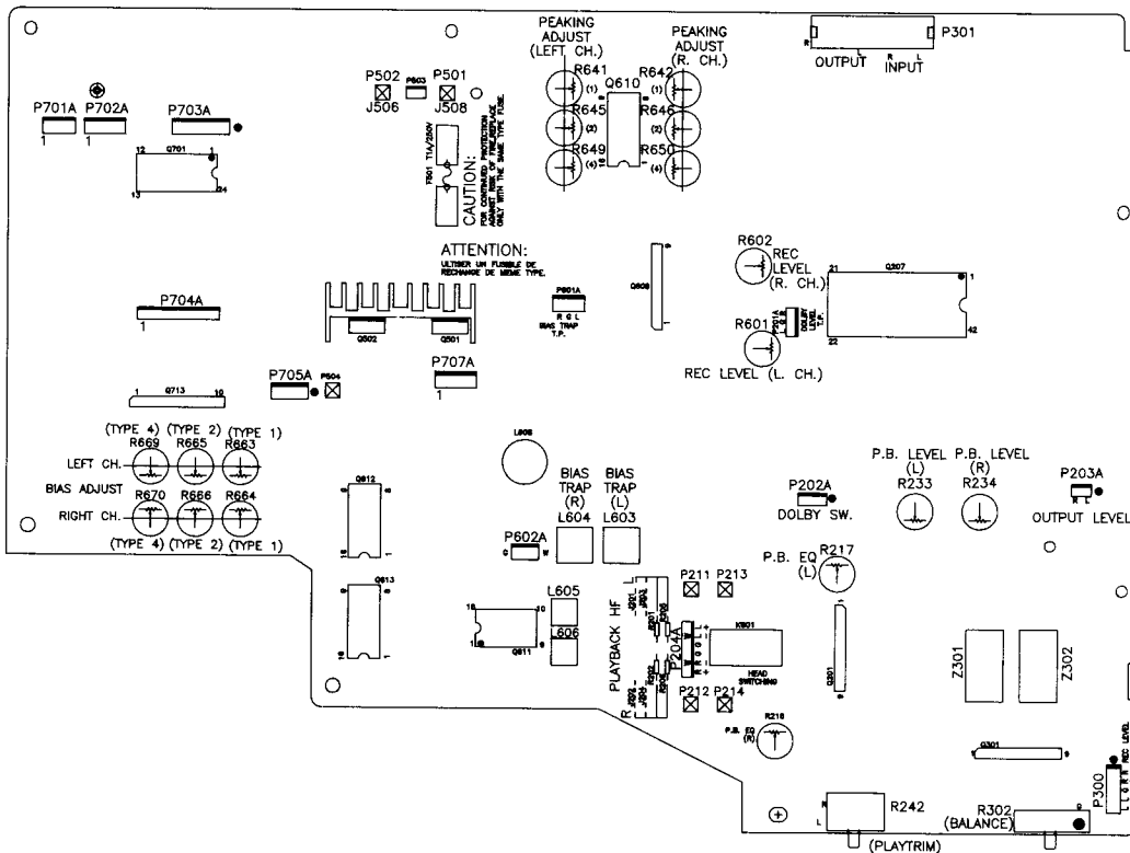
Fig. C FOR MAIN PCB
