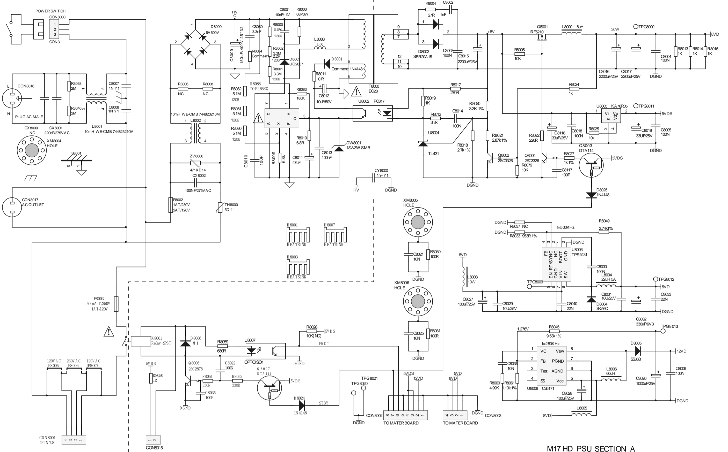
M17 HD PSU SECTION A
