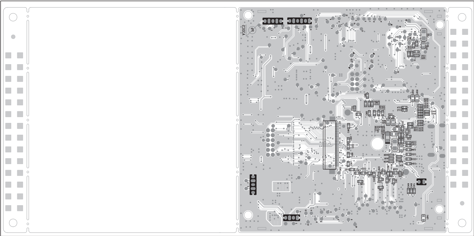
BOTTOM VIEW
