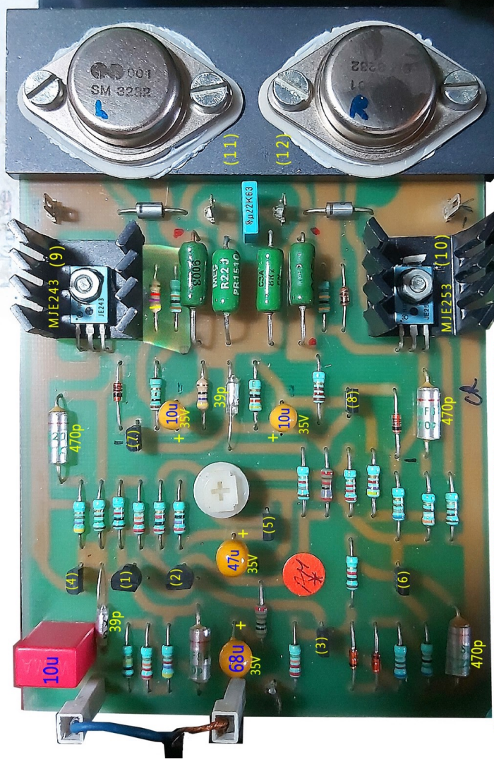
1,2=BC239(N) 3=MPSA06(N) 4=ZTX752(P) 5=ZTX384(N) 6=ZTX652(N) 7=MPSA06(N) 8=MPSA56(P) 9=MJE243(N) 10=MJE253(P) 11,12=NAIM001
