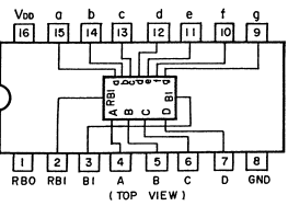
Fig. 13.20 BCD to 7-Segment Decoder/Driver C-MOS IC TC5022BP
