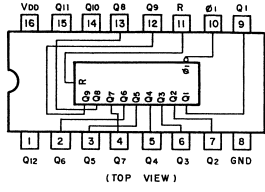
Fig. 13.21 12-Stage Binary Counter C-MOS IC TC4040BP
