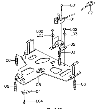
8.24. Cassette Case Holder L Ass'y (G05)
