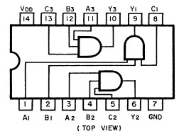
Fig. 13.15 AND Gate C-MOS IC μPD4073BC (TC4073BP)
