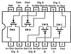
Fig. 13.6 Bilateral Switch C-MOS IC μPD4066C
