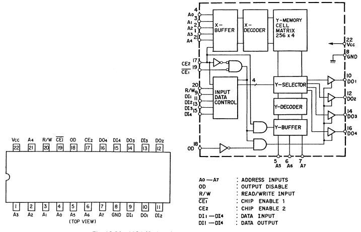
Fig. 13.26 1024 (256 x 4) Bit Static RAM IC μPD5101LC
