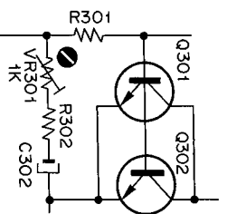
Fig. 4.6 Output Level
