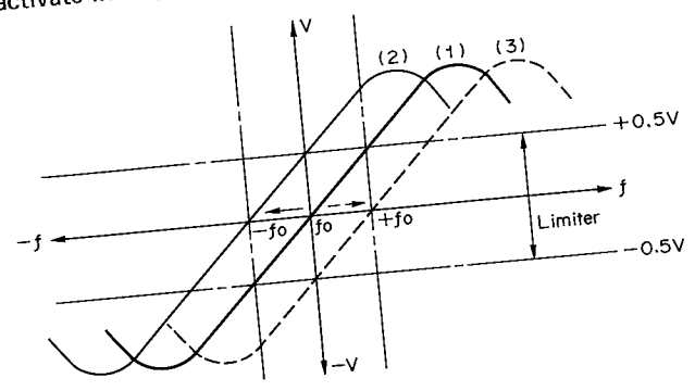
Fig. 2.6 S-Curve and AFC
