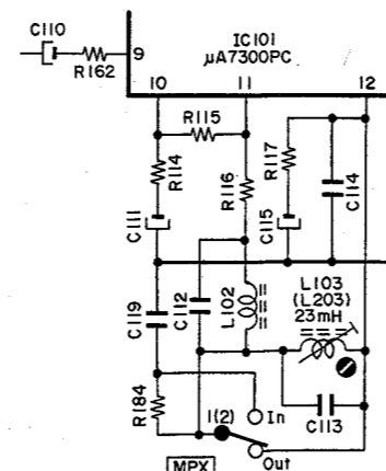
Fig. 7.2 3. MPX Filter
