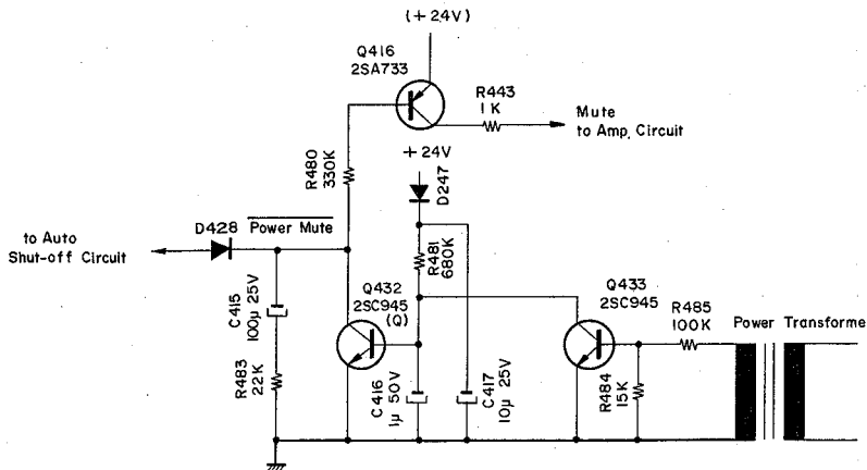
Fig. 2.3.3 Power-mute Circuit
