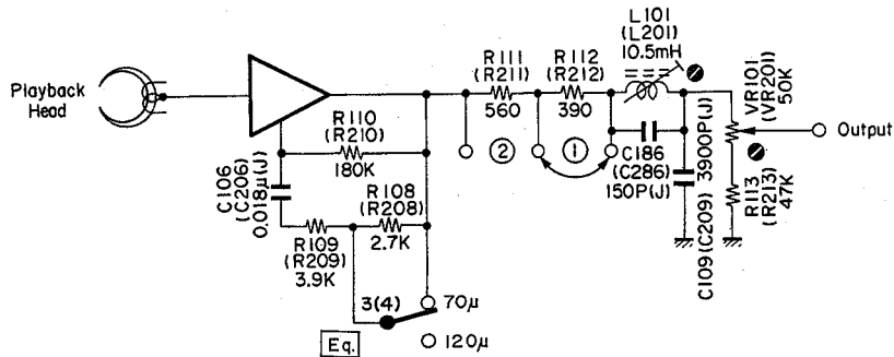
Fig. 2.2.2 System Diagram
