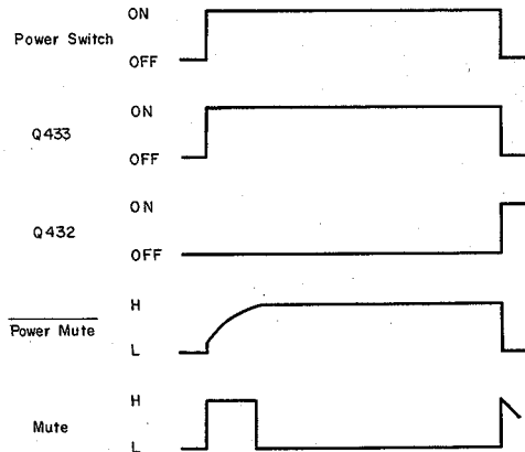
Fig. 2.3.4 Timing Chart
