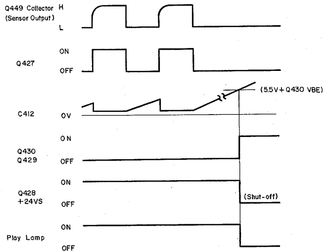
Fig. 2.3.6 Timing Chart
