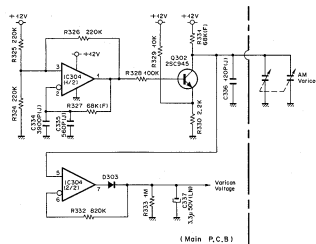
Fig. 2.3.5 Varicon Voltage Generating Circuit
