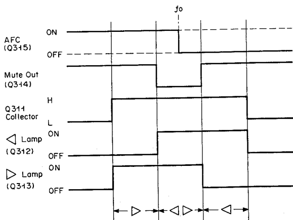
Fig. 2.3.14 Manual Preset Tuning Timing Chart
