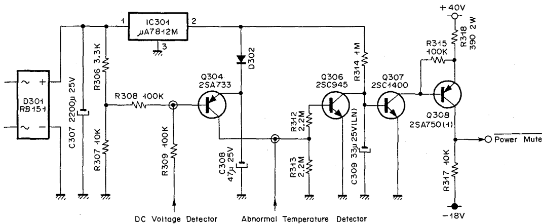
Fig. 2.2.2 Power Mute Generating Circuit
