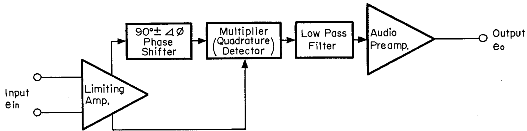
Fig. 2.1.16 Quadrature Detector System Diagram
