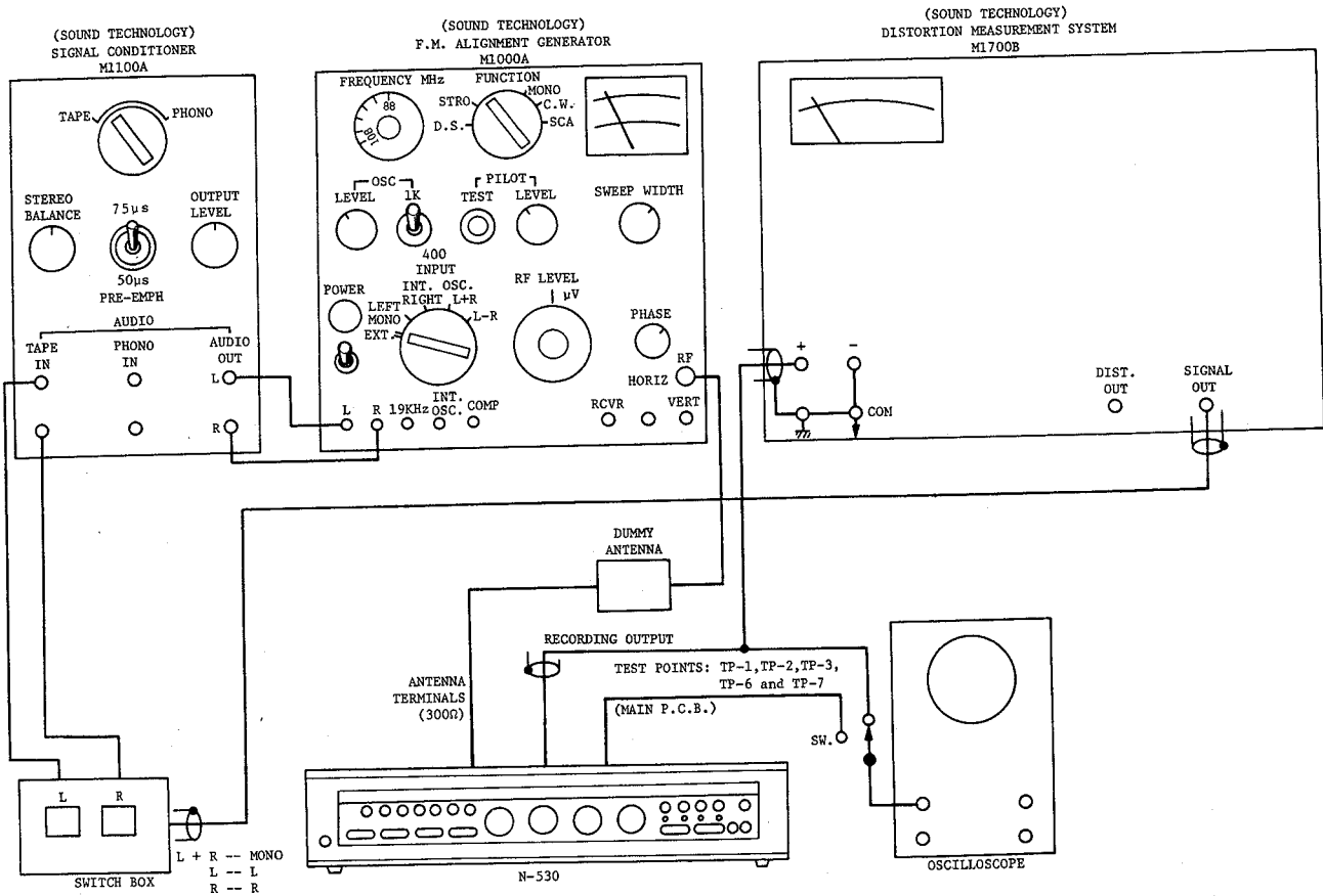
Fig. 4.1.2 Connection Diagram
