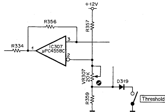
Fig. 4.1.10 11. Threshold Level
