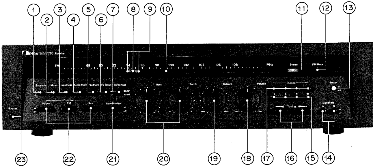
Fig. 1.1 Front View
