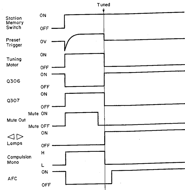
Fig. 2.3.15 Auto-Preset Tuning Timing Chart
