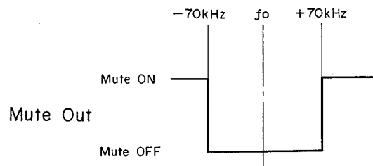
Fig. 2.3.13 Mute Out Signal
