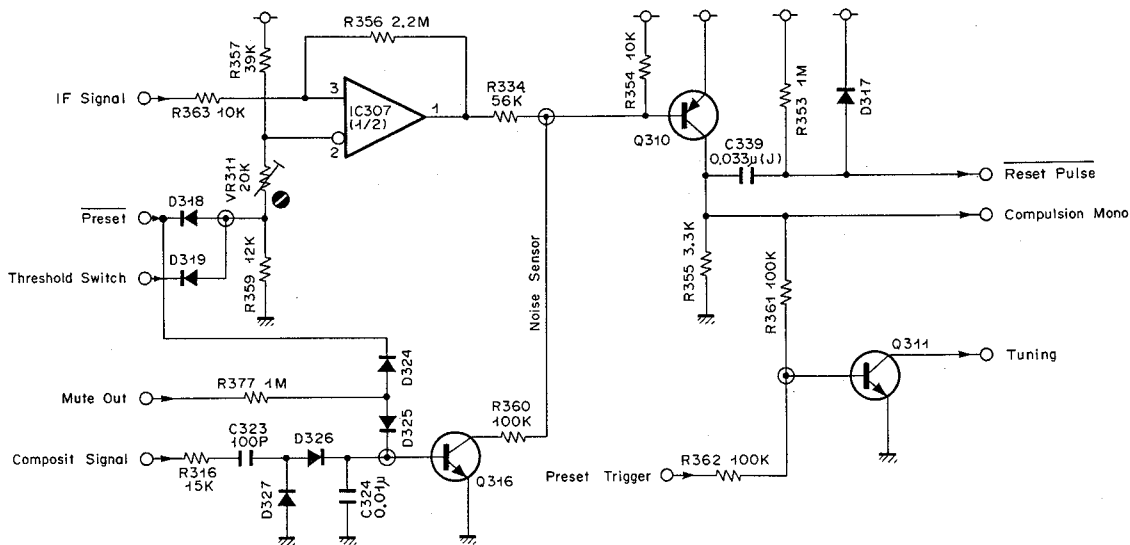
Fig. 2.3.10 Station Detecting Circuit
