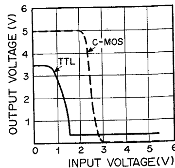
Fig. 2.1.2 Input-Output Transmission Characteristics
