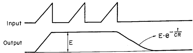
Fig. 2.1.15 Timing Chart
