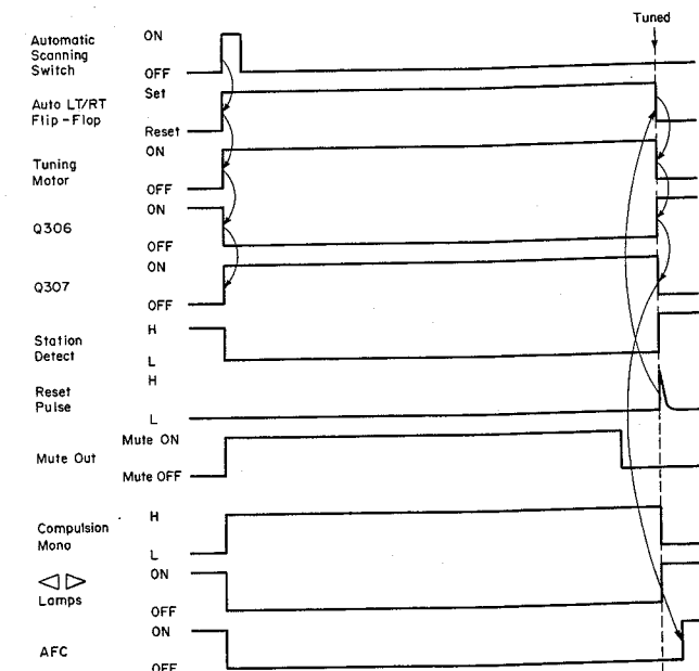
Fig. 2.3.16 Auto-Tuning Timing Chart
