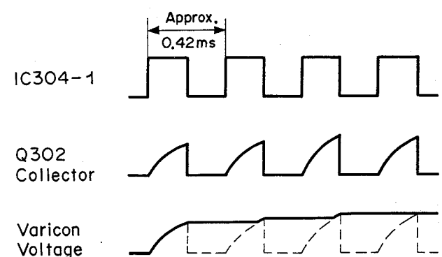
Fig. 2.3.6 Timing Chart
