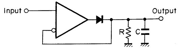
Fig. 2.1.14 Peak Holding Circuit
