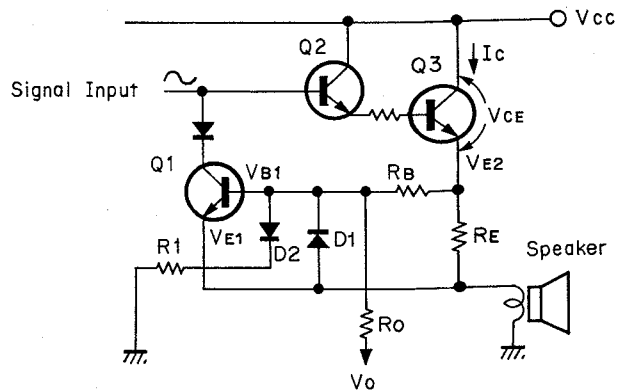
Fig. 2.4.12 Limiter Circuit
