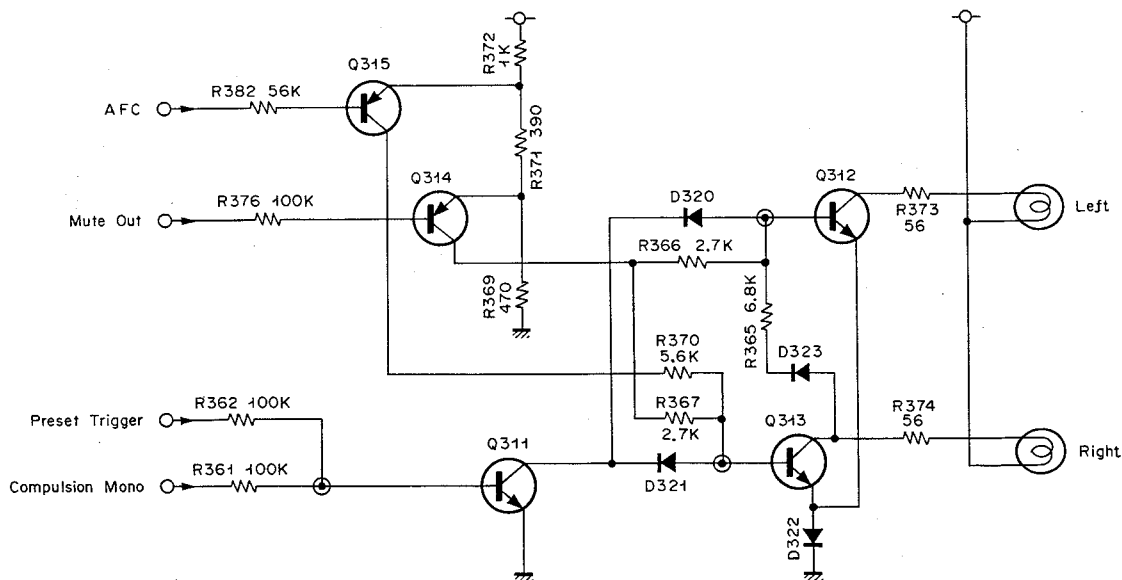
Fig. 2.3.12 Tuning Indicator Control Circuit
