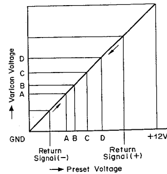
Fig. 2.3.8 Preset Voltage Range
