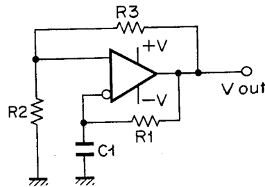
Fig. 2.1.12 Oscillator
