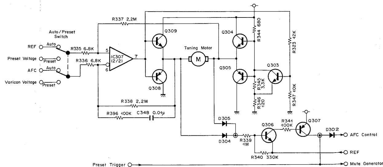
Fig. 2.3.7 Motor Drive Circuit and Frequency Sensor Circuit
