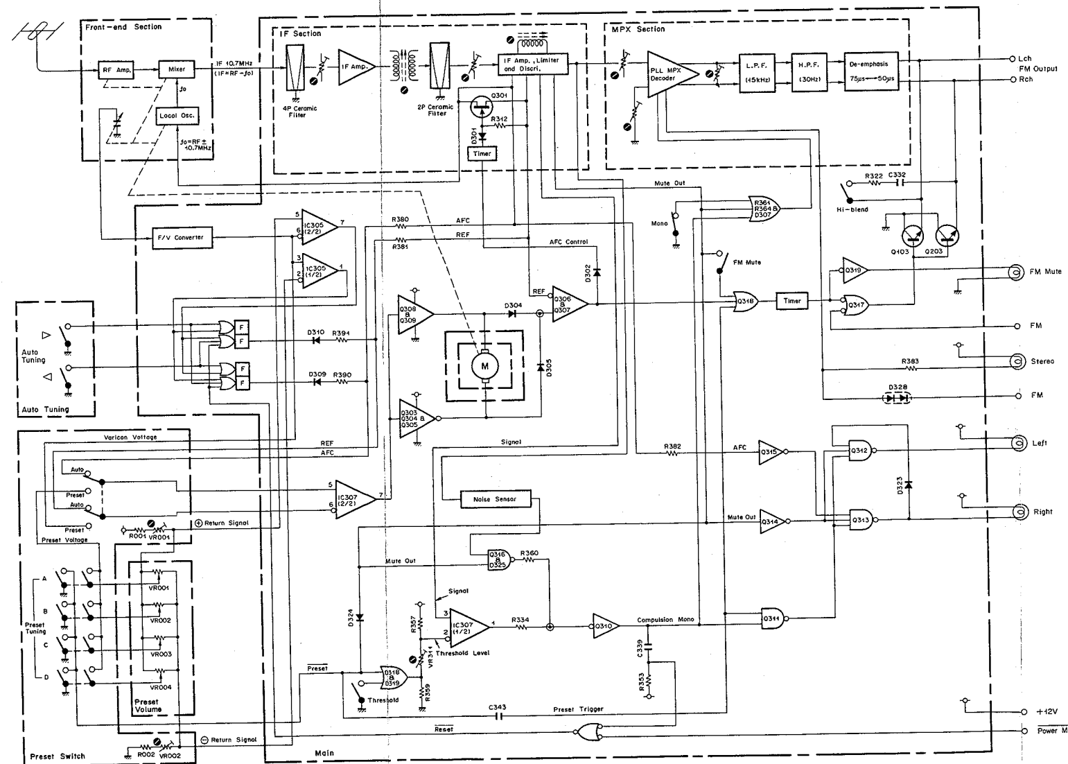
Fig. 2.3.3 FM Tuner System Diagram
