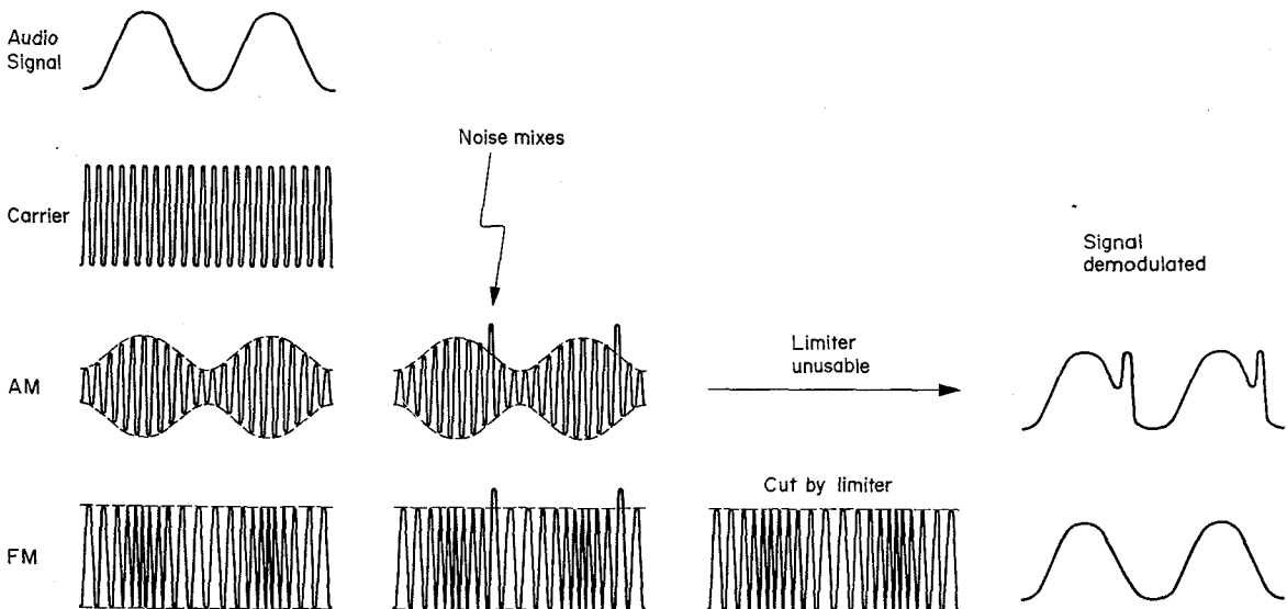
Fig. 2.3.1 AM and FM
