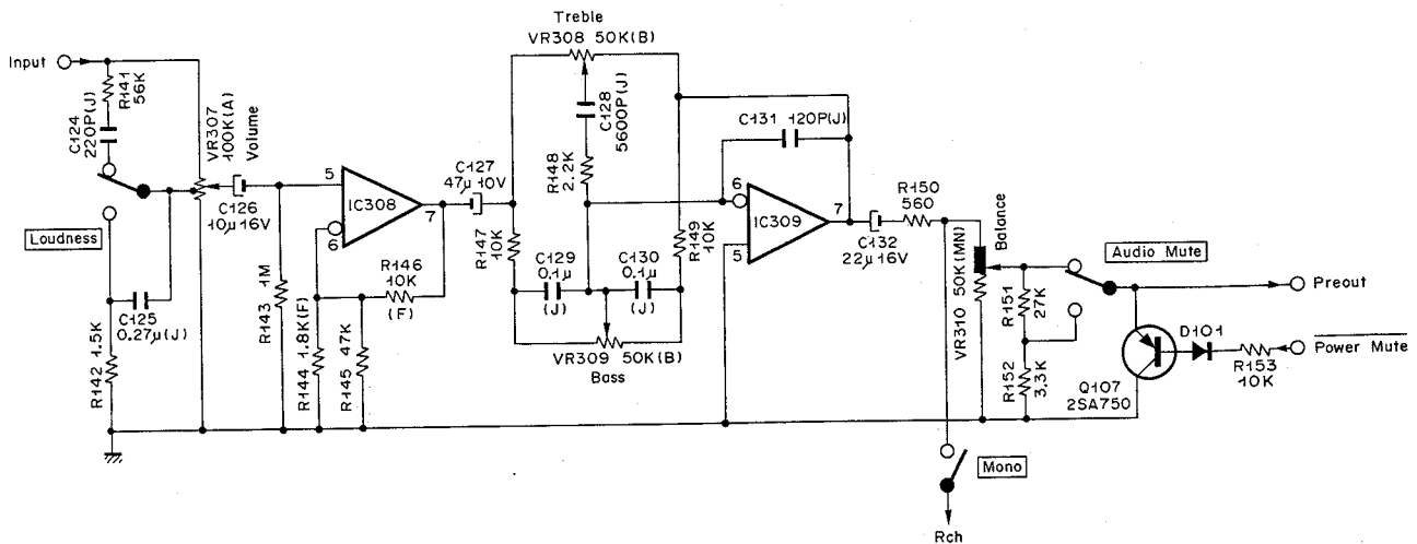
Fig. 2.4.5 Tone Control Circuit
