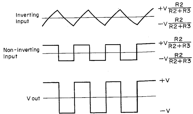
Fig. 2.1.13 Timing Chart
