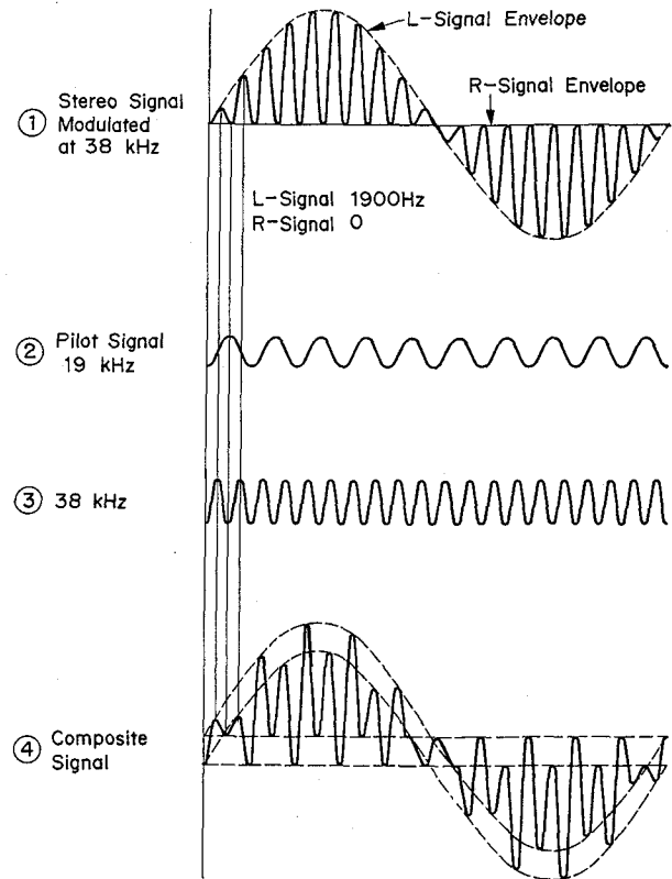
Fig. 2.3.2 MPX Stereo Signal
