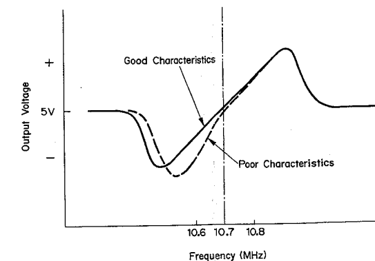
Fig. 2.3.4 Discriminator Characteristics (S-Curve)
