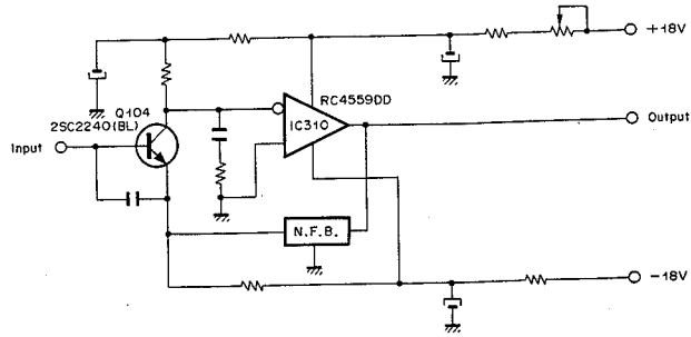
Fig. 2.4.1 Phono Eq. Amp. Circuit
