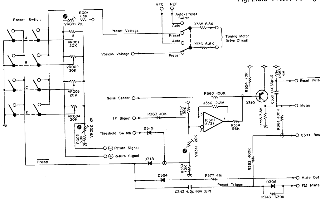
Fig. 2.3.9 Preset Tuning Circuit
