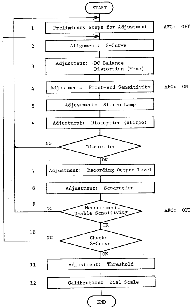
Fig. 4.1.1 Adjustment Flow Chart
