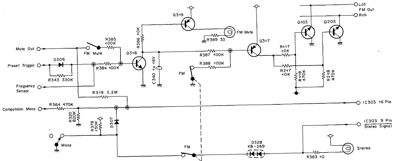
Fig. 2.3.17 FM Mute and Compulsion Mono Circuit
