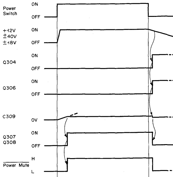
Fig. 2.2.1 Power Mute Timing Chart
