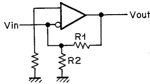
Fig. 2.1.11 Inverting
