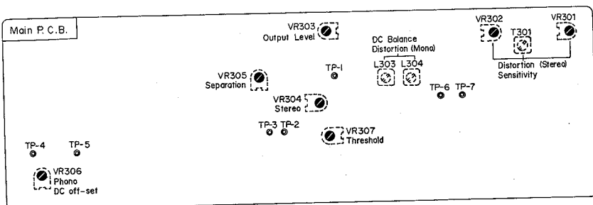
Fig. 4.1.3 Diagram for Adjustment
