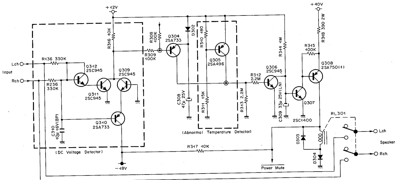
Fig. 2.4.13 Protector Circuit
