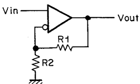
Fig. 2.1.10 Non-inverting
