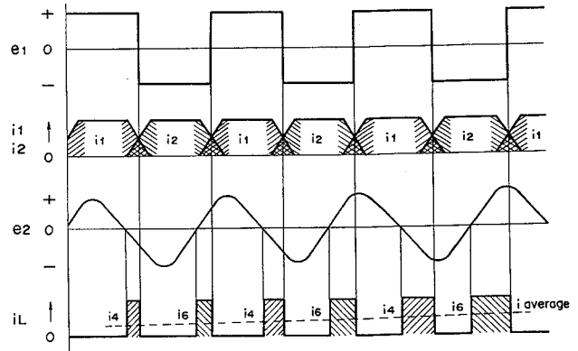
Fig. 2.1.18 Timing Chart
