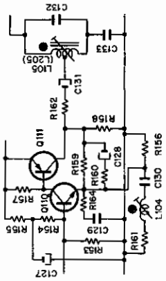
Fig 6.1.7 Bias Osc. Frequency
