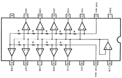
FIG. 8.1.4 Level Meter Driver TA7612AP
