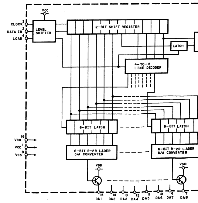
Fig. 8.1.16 μPD6326C-028
