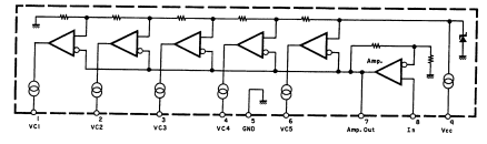
Fig. 7.1.13 Signal Meter Driver IC LB1413N
