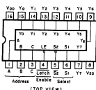
Fig. 7.1.6 3-to-8 Line Decoder IC \mu PD74HC237
