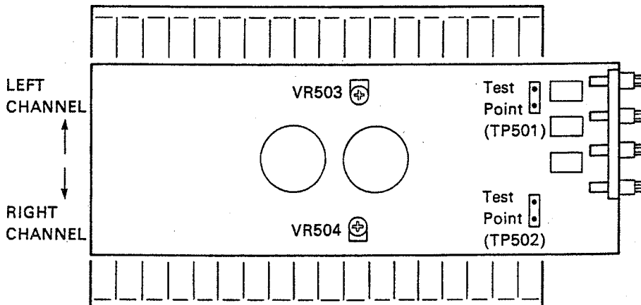
Figure 2 Adjustment Points
