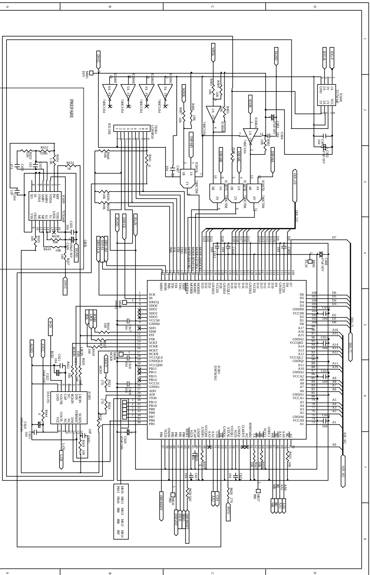
DSP SCH DRAM AND FLASH ROM NEW ADDRESS DSP ICE 9P
