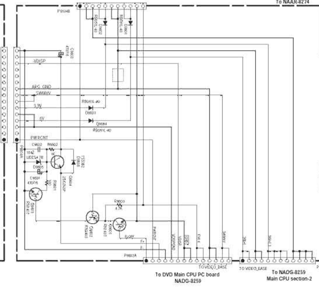
U13 : POWER SUPPLY PC BOARD-2 NAPS-8270
