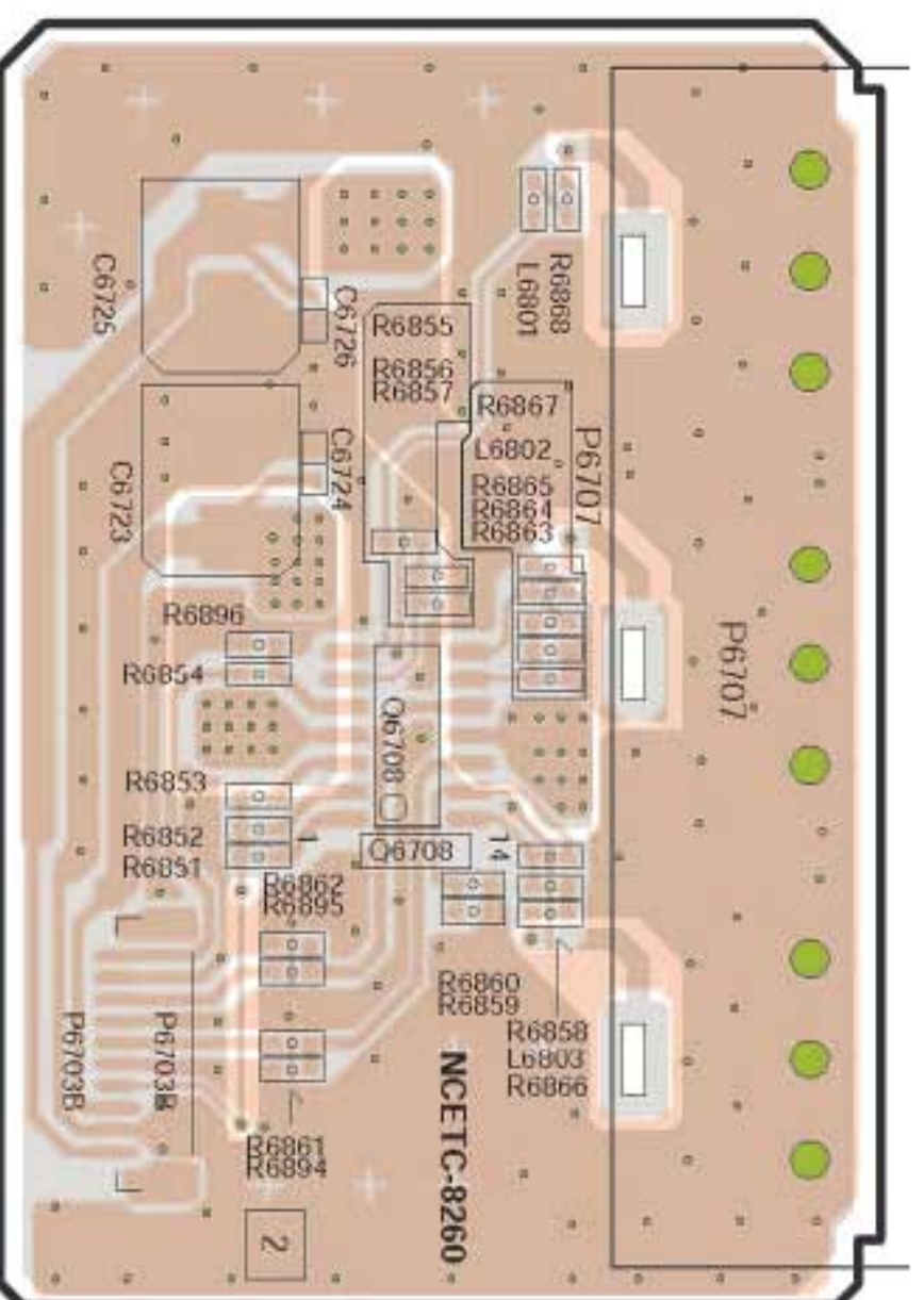
B-SIDE VIEW
