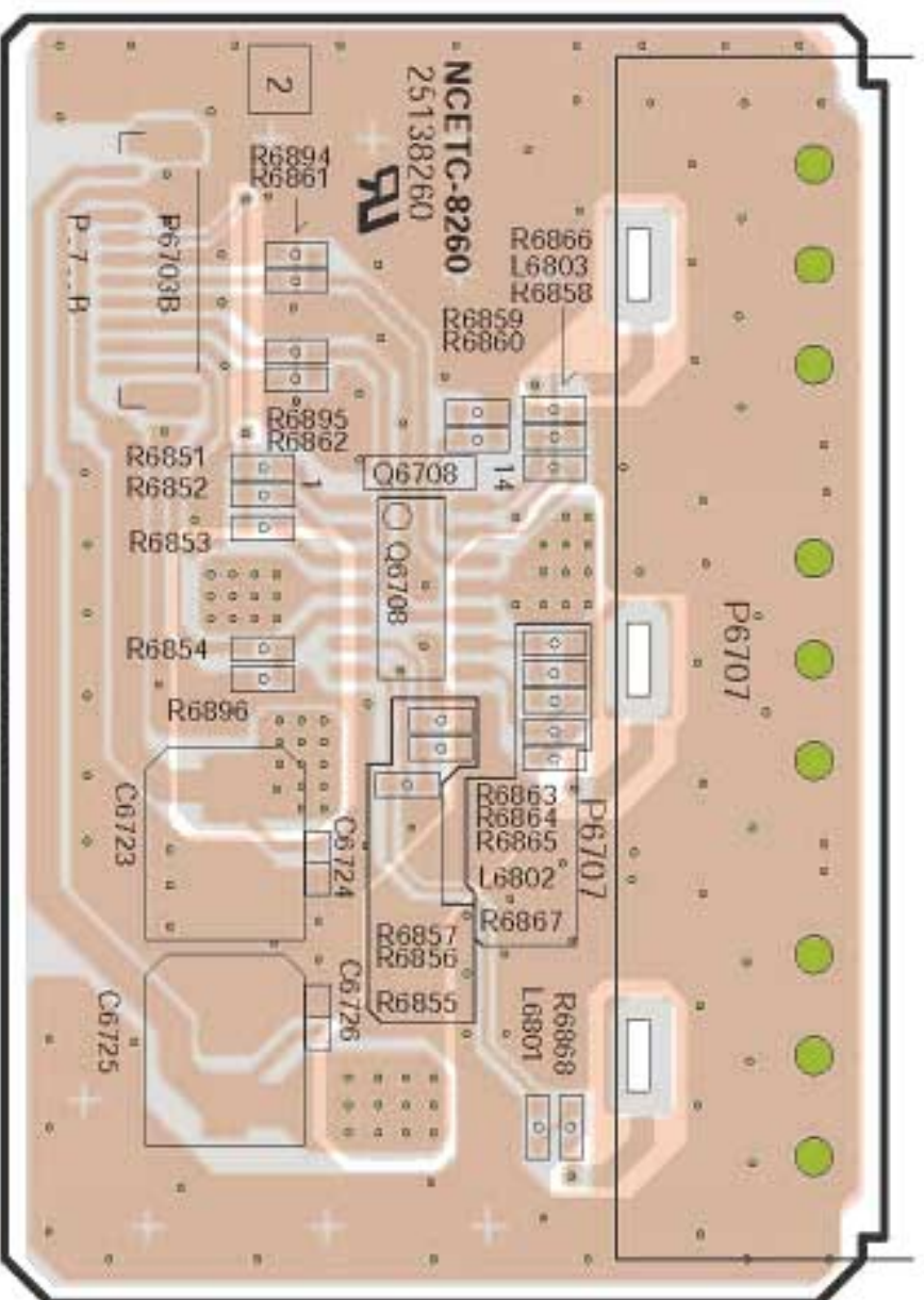
A-SIDE VIEW
