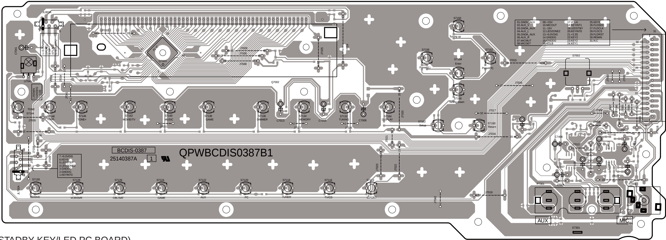
BADIS-0388 (STADBY KEY/LED PC BOARD) A-side(Component side)
