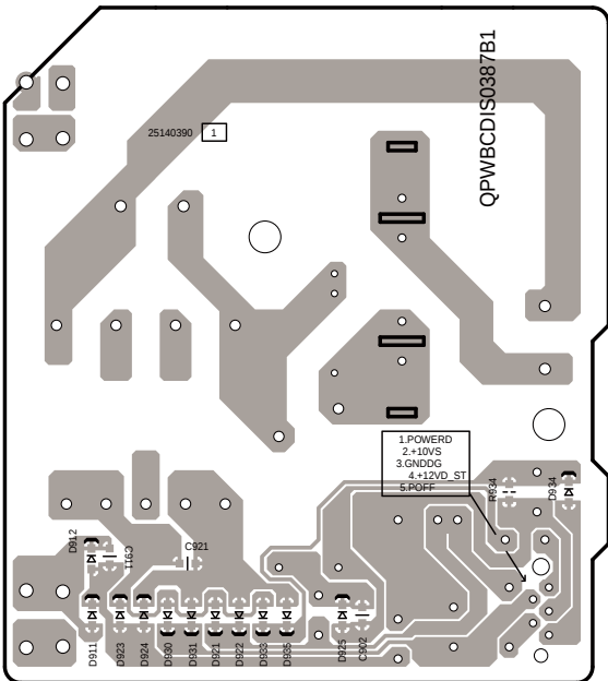
BAETC-0390 (POW SUPPLY PC BOARD) B-side(Soldering side)
