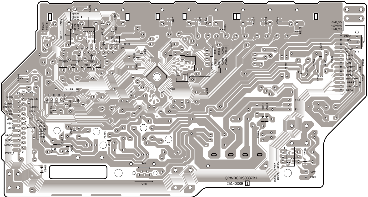
BADIS-0389 (VIDEO PC BOARD) B-side(Soldering side)
