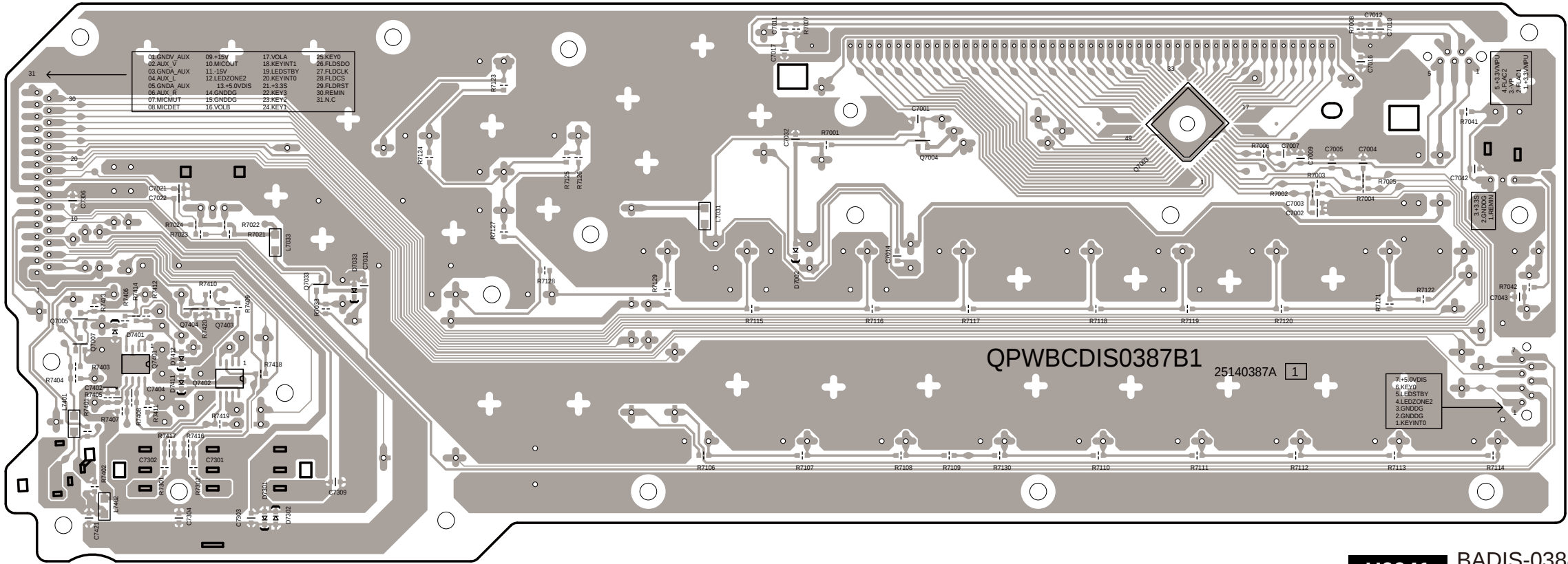
BADIS-0389 (VIDEO PC BOARD) B-side(Soldering side)
