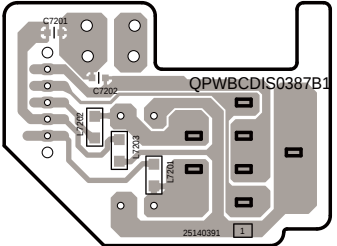
BAETC-0391 (HP JACK PC BOARD) B-side(Soldering side)
