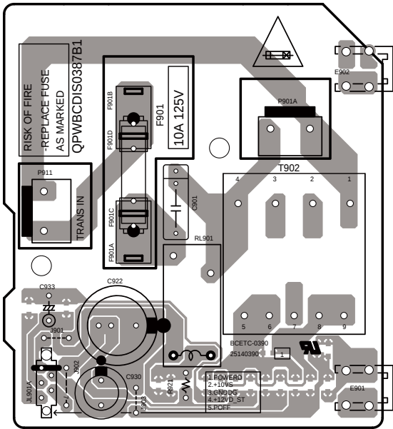
BAETC-0390 (POW SUPPLY PC BOARD) A-side(Component side)
