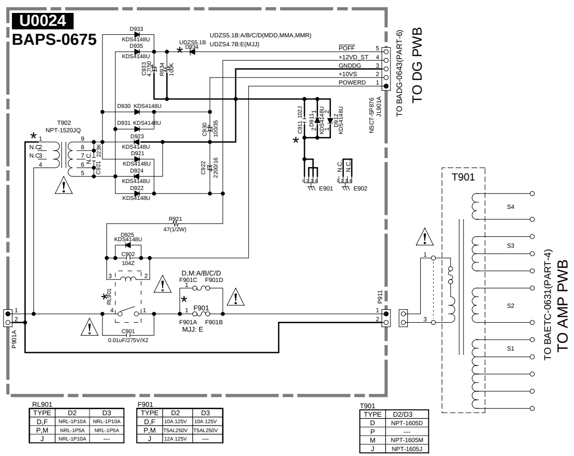
Model No. DTR-20.3/DTR-30.3 Schematic Diagram (Part-10) PS Section
