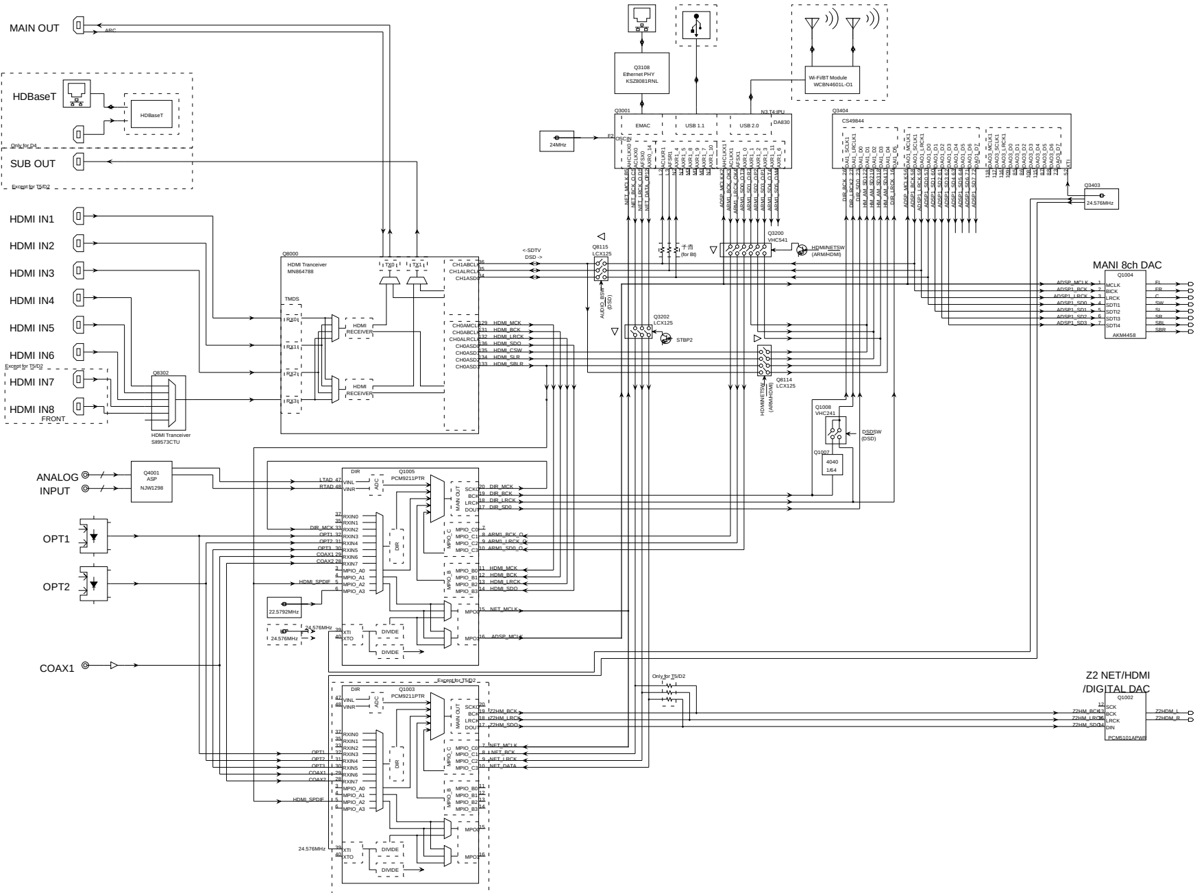
MODEL NO.TX-NR545/646/747,DTR-20.7/30.7/40.7 SCHEMATIC DIAGRAM (PART-3) BLOCK DIAGRAM(Digital Aud
