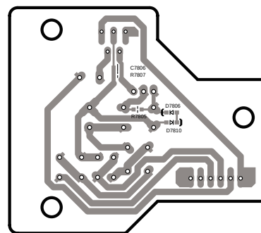
Sodering side view from component side
