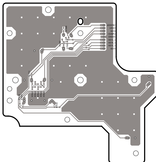
Sodering side view from component side
