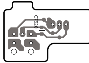
Soldering side view from component side
