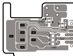
Sodering side view from component side
