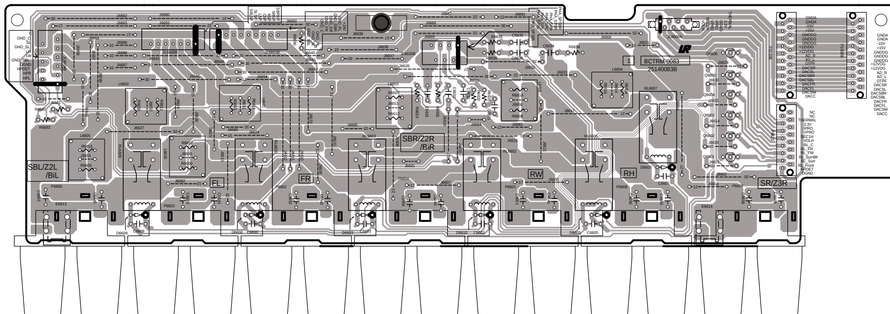
Soldering side view
