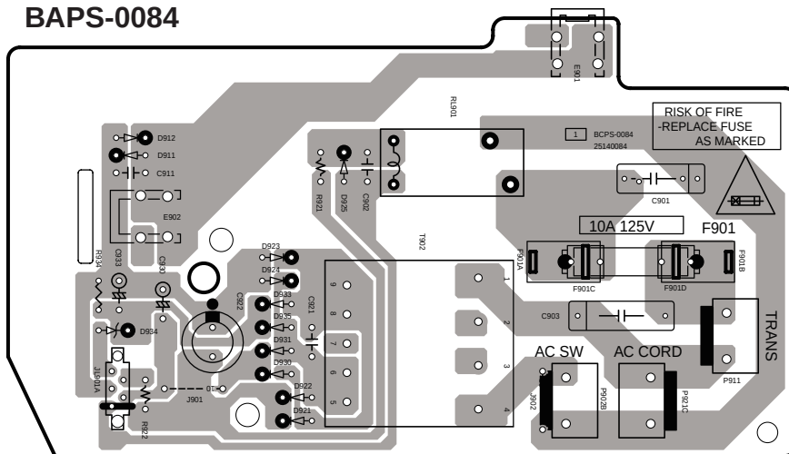
Soldering side view
