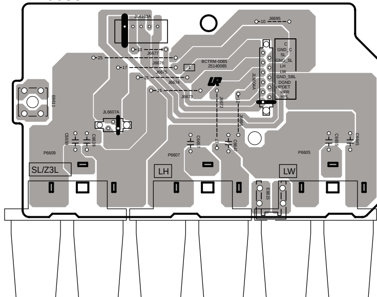
Soldering side view
