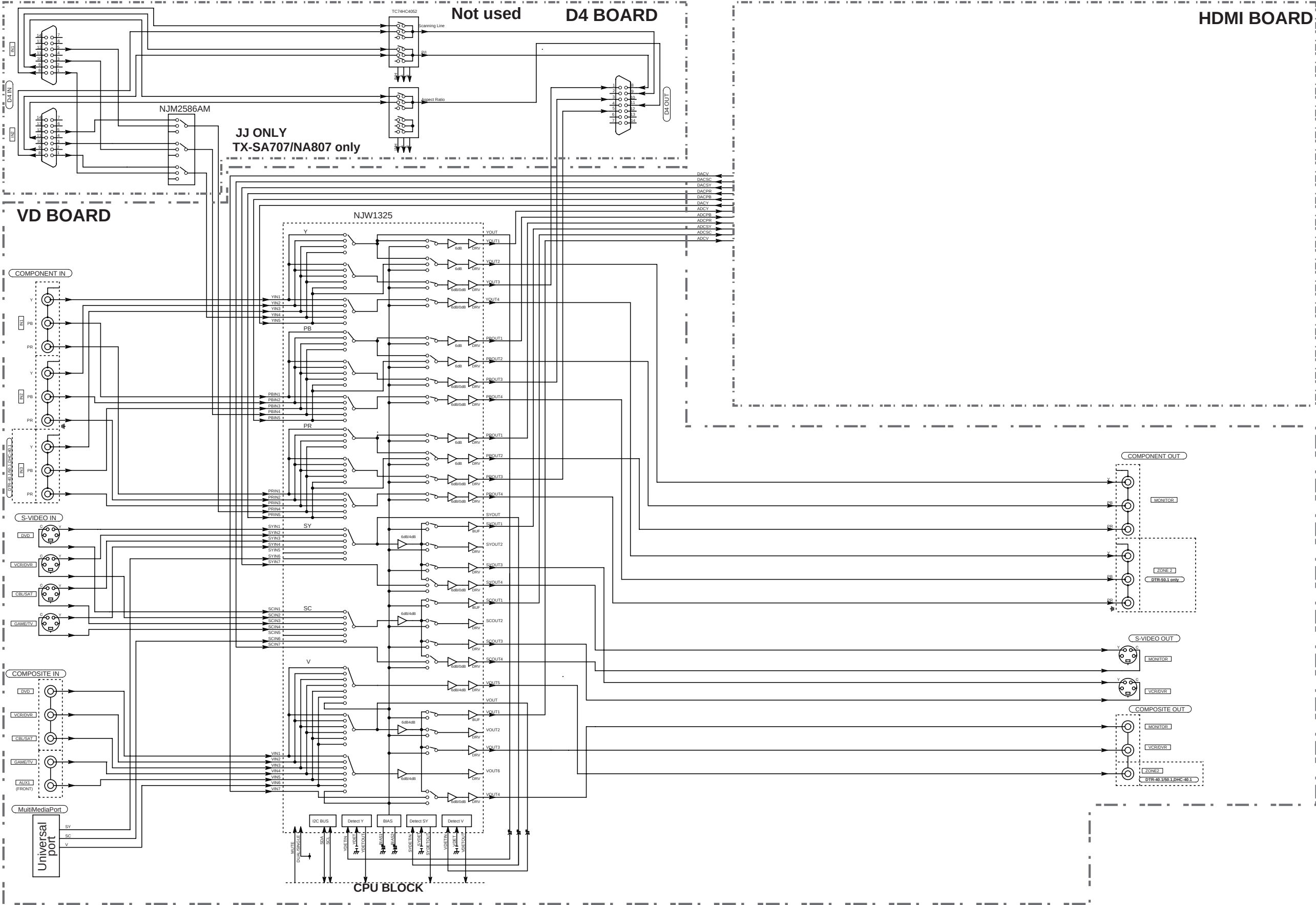
BLOCK DIAGRAM-2
