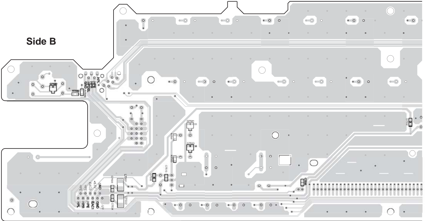
NADIS-8406 Display circuit PC board
