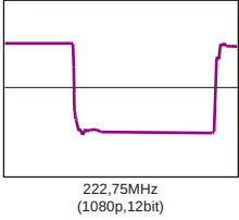
HDMI CK waveform (WF42) PART-11:B3, H4
