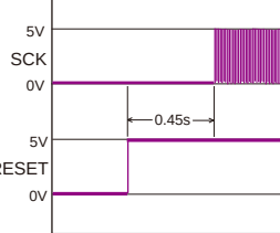
SCK/RESET waveform (WF63) PART-9:F4/D4
