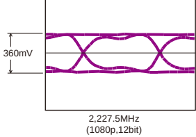
HDMI D0,D1,D2 waveform (WF41) PART-11:B3, H4
