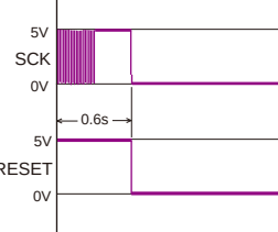
SCK/RESET waveform (WF63) PART-9:F4/D4
