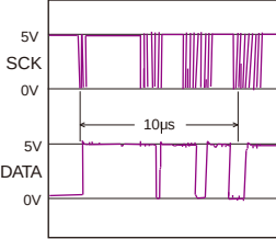
SCK/SDATA waveform (WF61) PART-9:F4/D4
