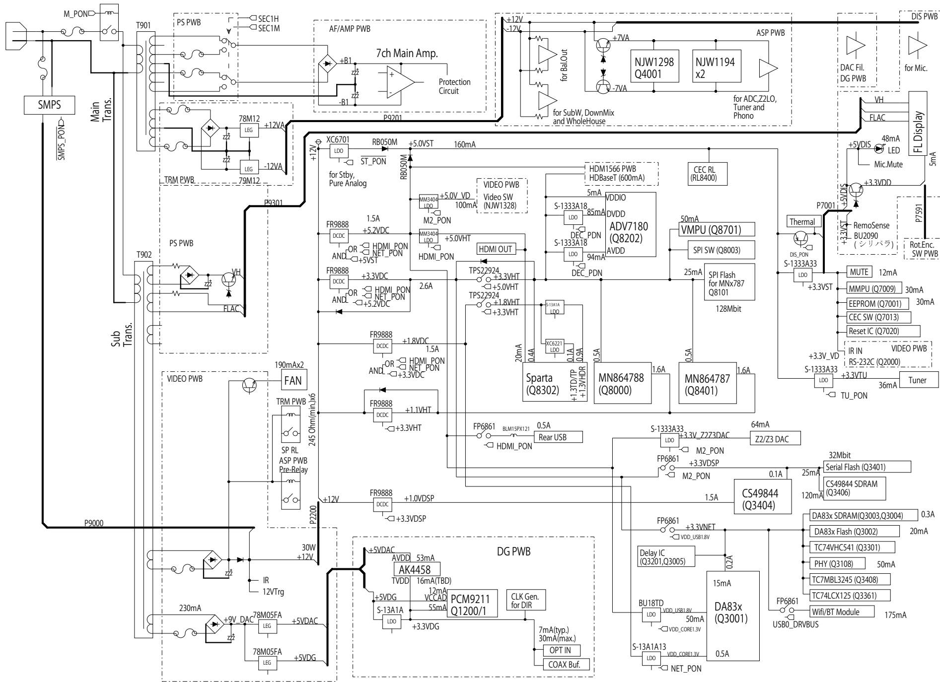
Block Diagram (Power Section)
