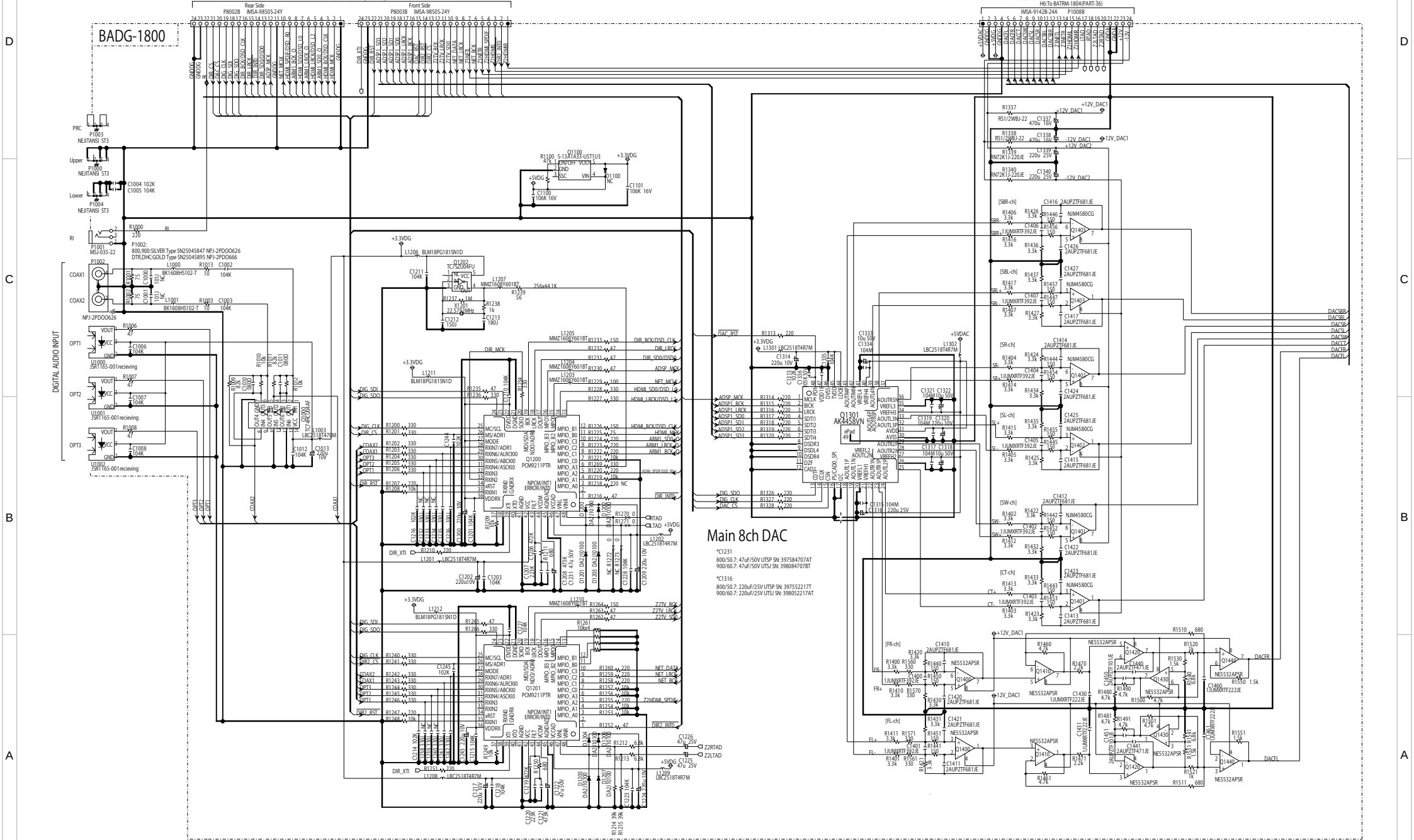
MODEL No. TX-RZ-800,900 DTR-50.7,60.7 DHC-60.7 SCHEMATIC DIAGRAM (PART-13)
