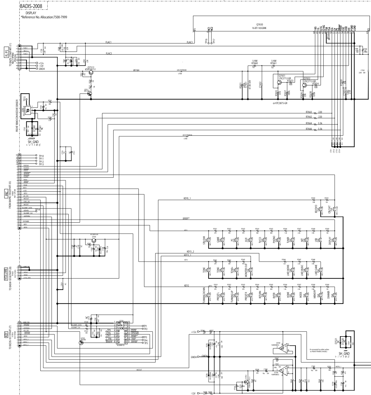
MODEL NO. DTR-50.8 SCHEMATIC DIAGRAM (PART-26) DISPLAY SECTION
