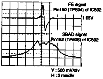
DVD single (single-layer) disc detection waveform
