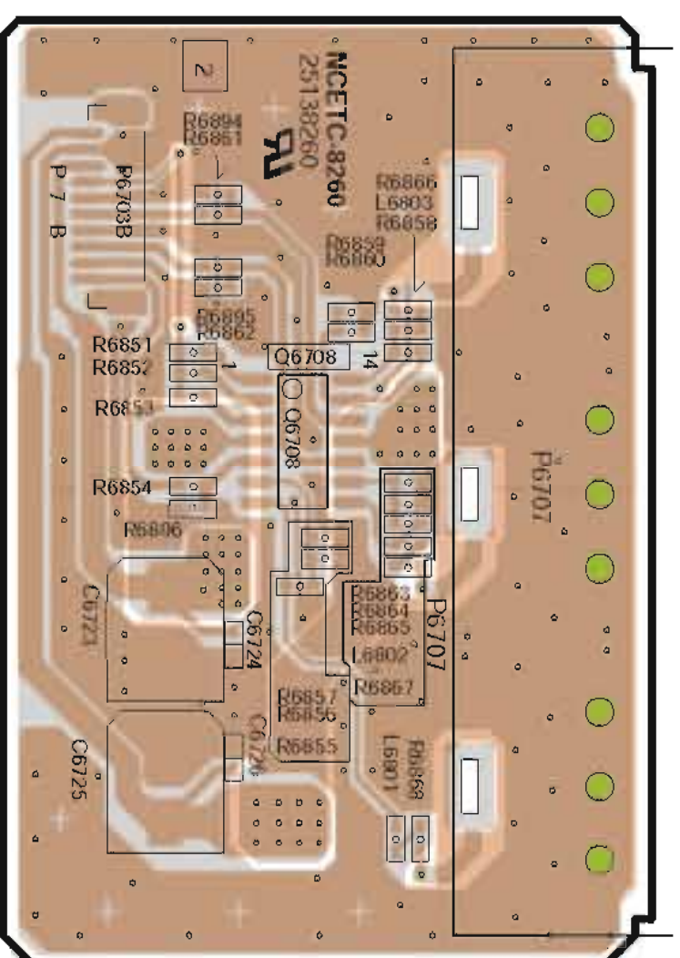
A-SIDE VIEW
