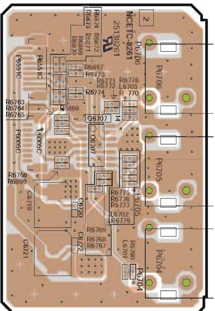
A-SIDE VIEW
