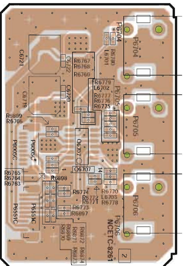
B-SIDE VIEW
