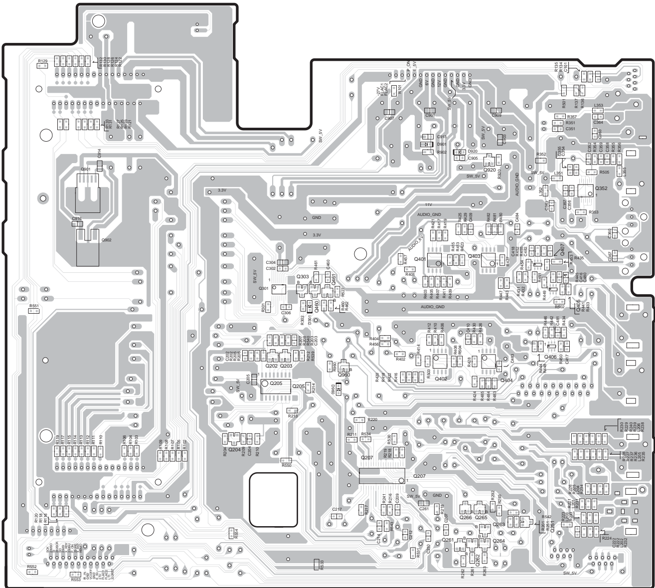
Soldering side
