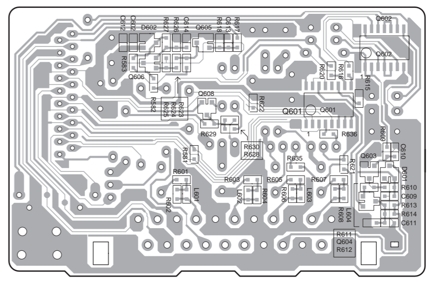
Soldering side view
