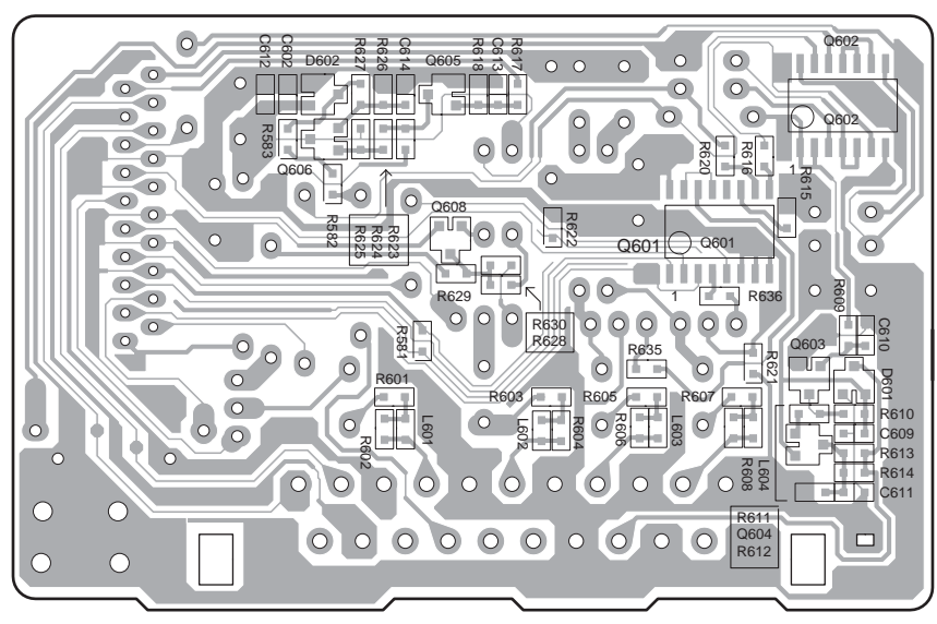
Soldering side view
