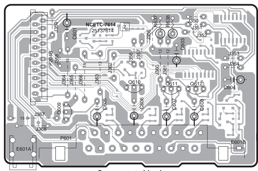
Component side view
