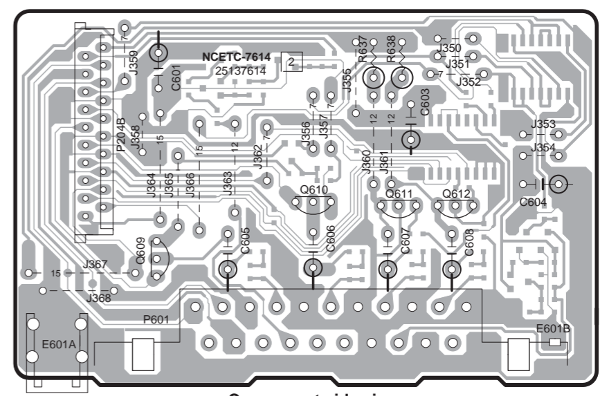
Component side view
