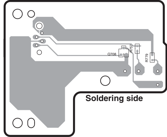
U3: STANDBY SWITCH PC BOARD NADIS-7999
