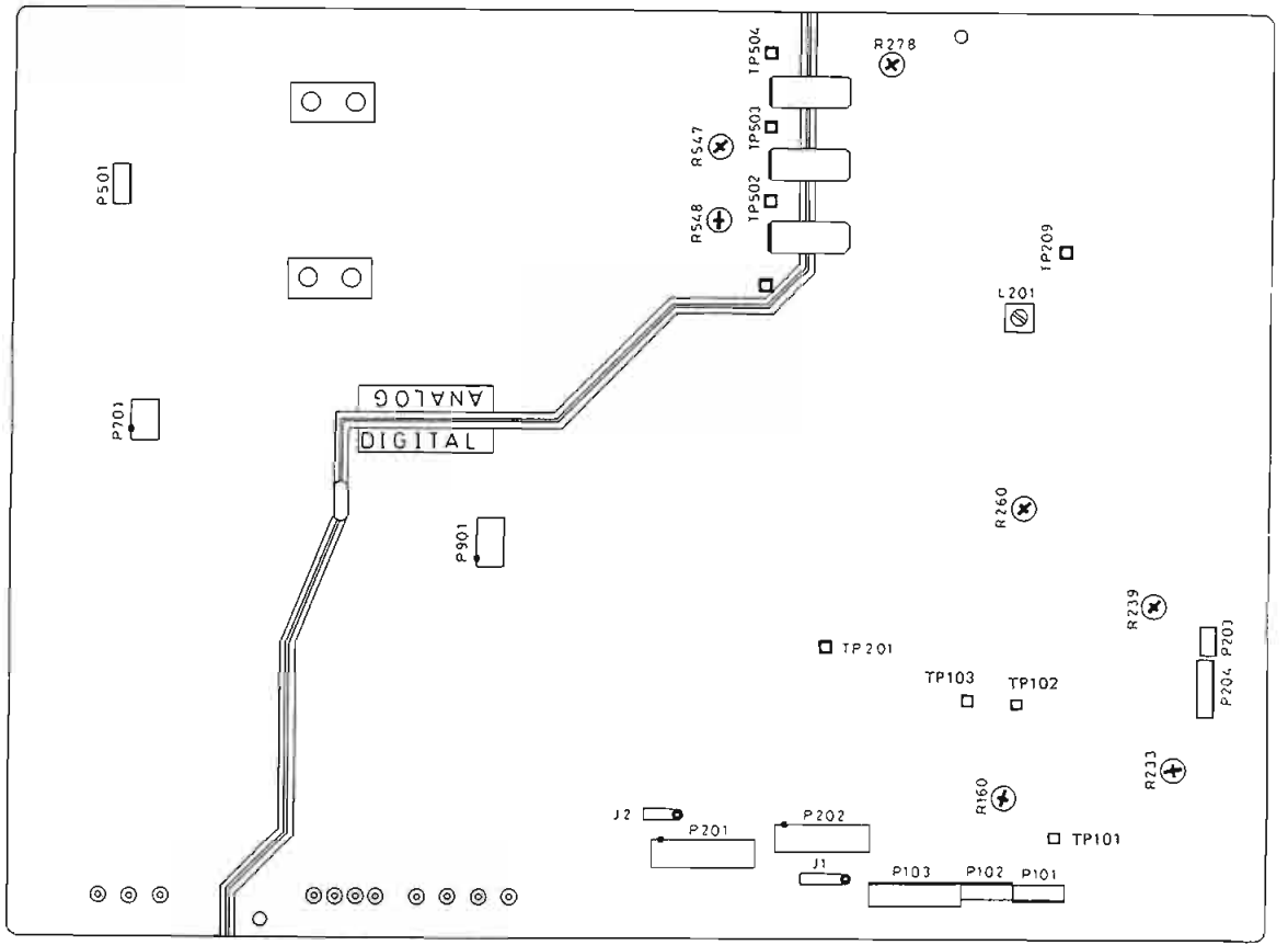
Fig. 60 Adjustment Point
