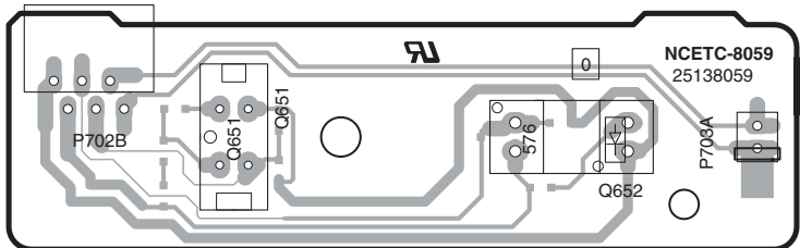
Component side
