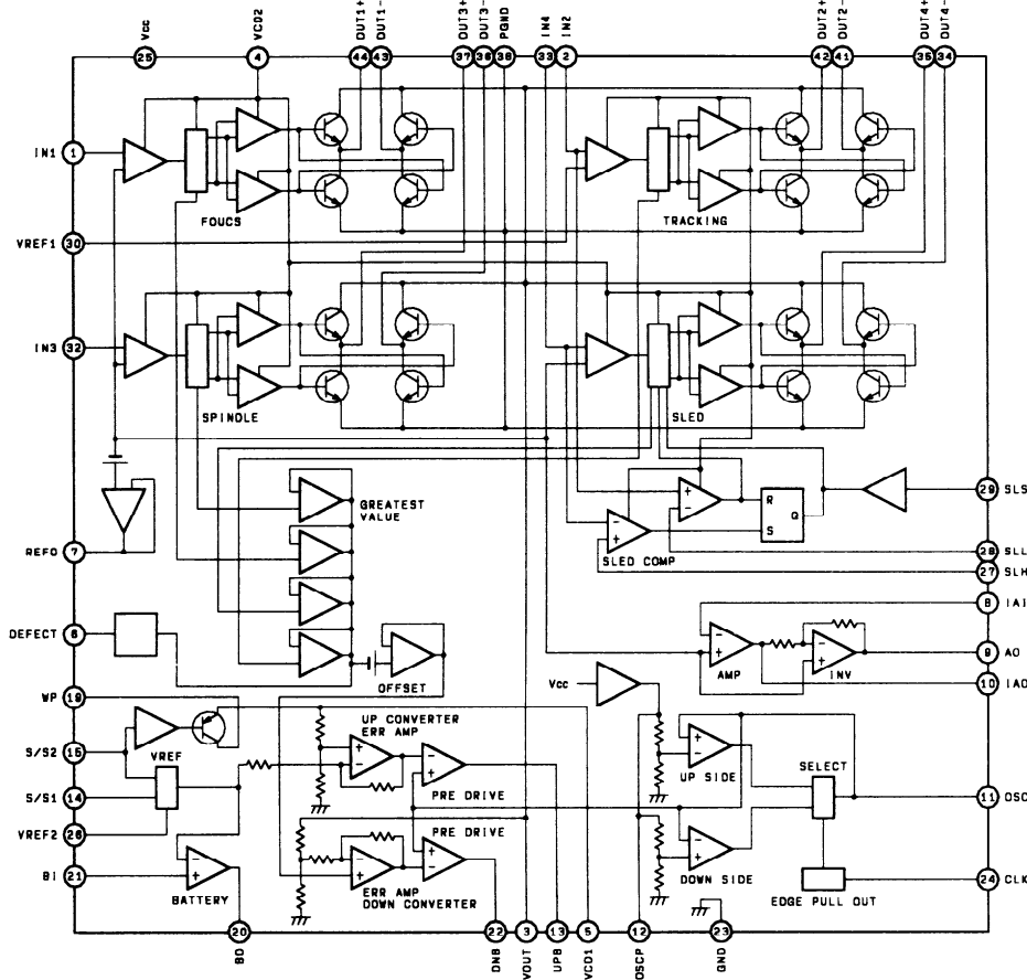
IC502 LB8106M BLOCK DIAGRAM (Focus Tracking Motor Driver)
