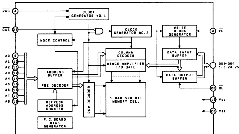
IC603 MB81C4256A-80PJ-G-LV BLOCK DIAGRAM (1M-DRAM)
