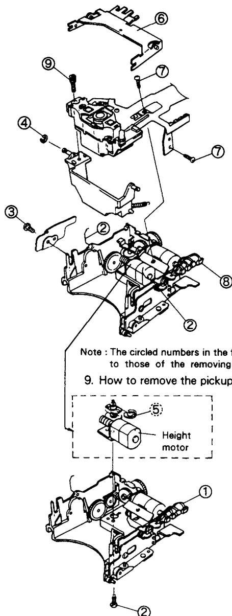
Fig. 7-16 How to remove the height motor
