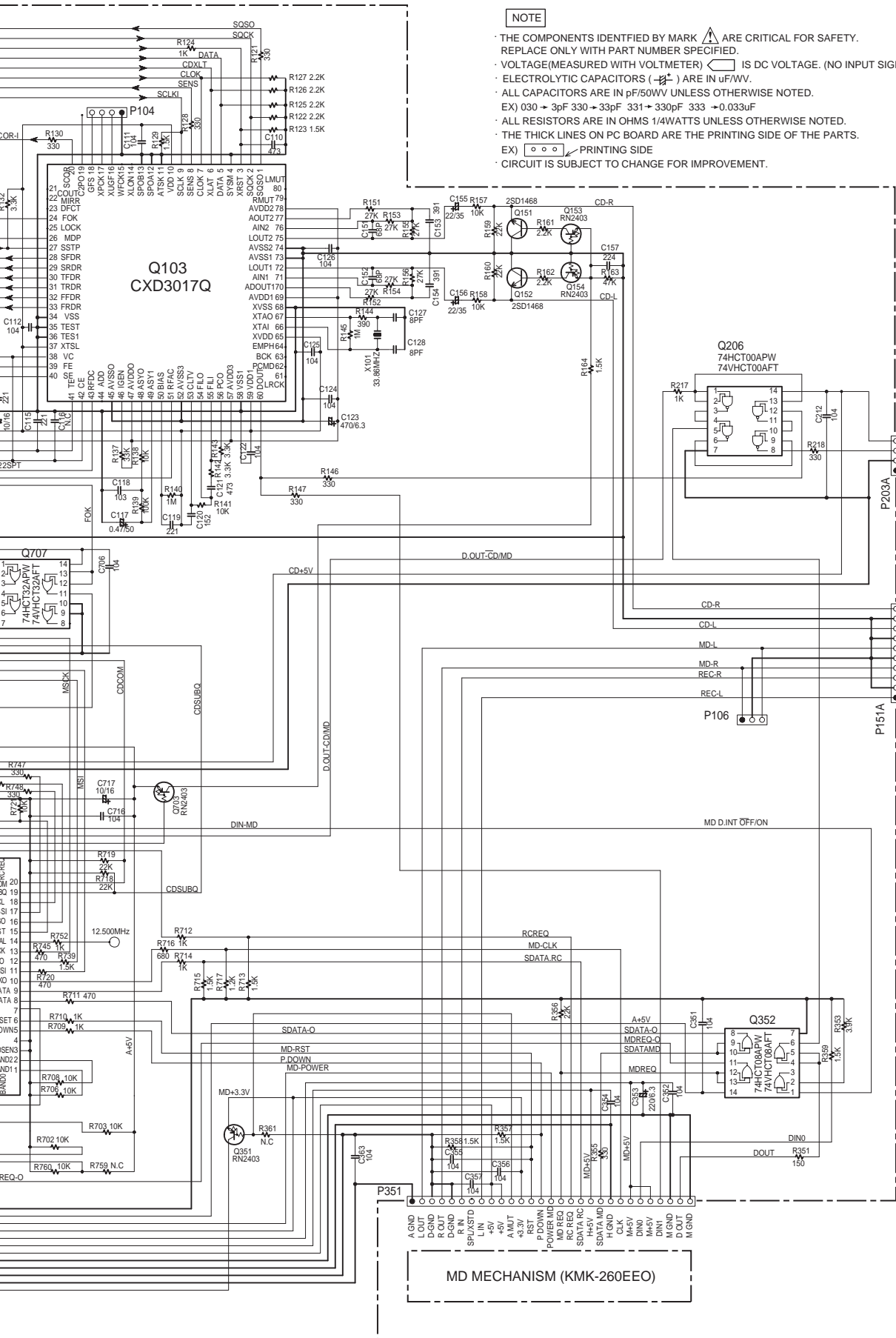
SCHMATIC DIAGRAMS-1 To NAAF-7585(P151B)
