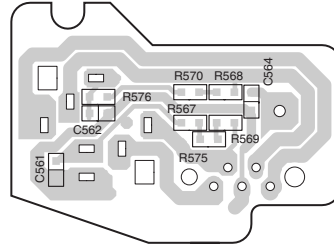
Soldering side
