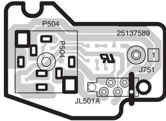
Component side
